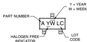
Micro3 / SOT-23 Package Marking
