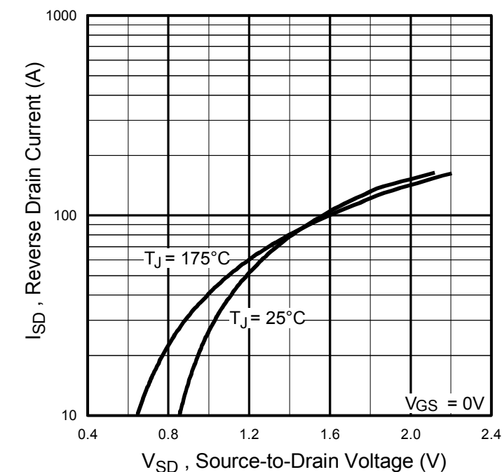
Fig. 7 Typical Source-to-Drain Diode Forward Voltage
