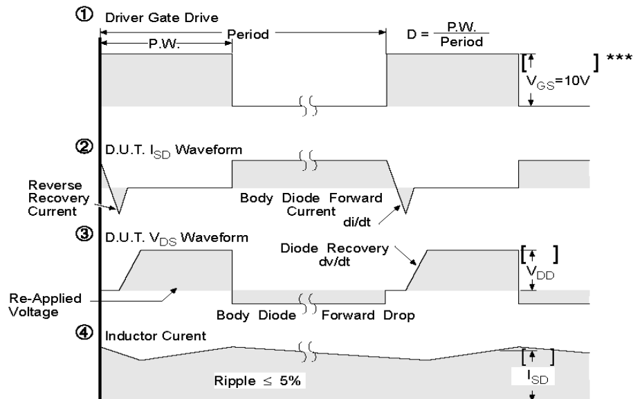
Fig 12. For P-Channel HEXFETS
