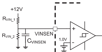
Figure 11: VINSEN resistor divider network
