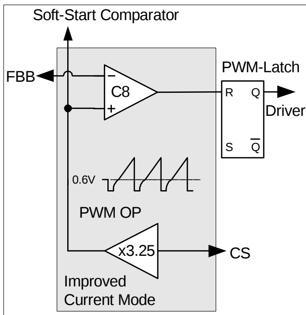
Figure 4 Current Mode
