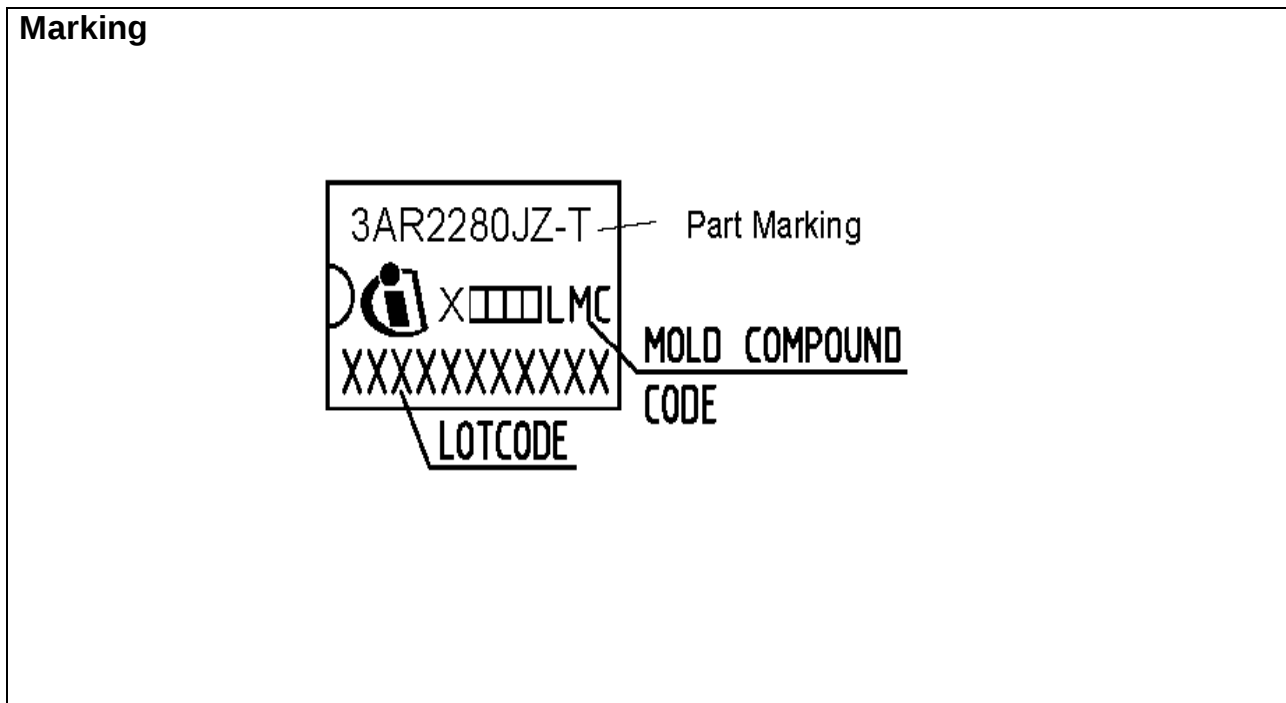
Figure 40 Marking for ICE3AR2280JZ-T
