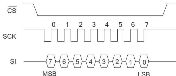
Figure 16. SPI Mode 3
