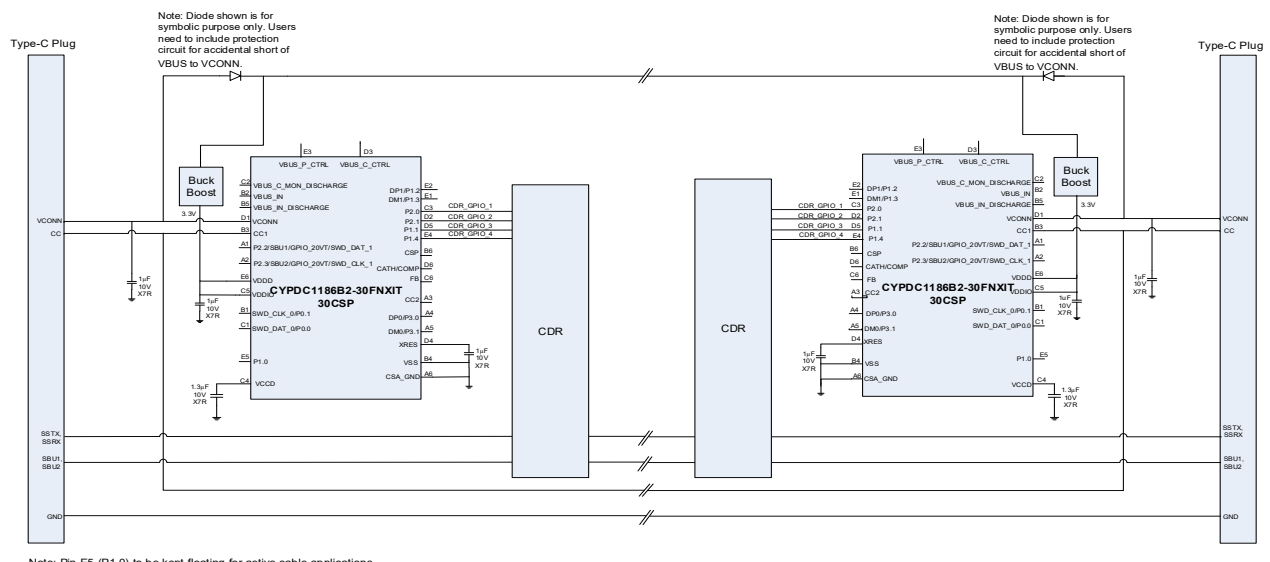
Figure 6. Thunderbolt™ Active Cable Application Diagram (Two Chips Per Cable) (For Silicon Rev = B2)
