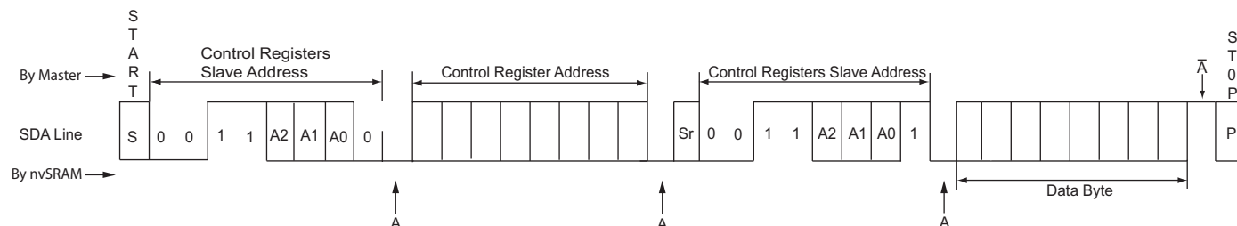
Figure 26. Random Control Registers Single-Byte Read
