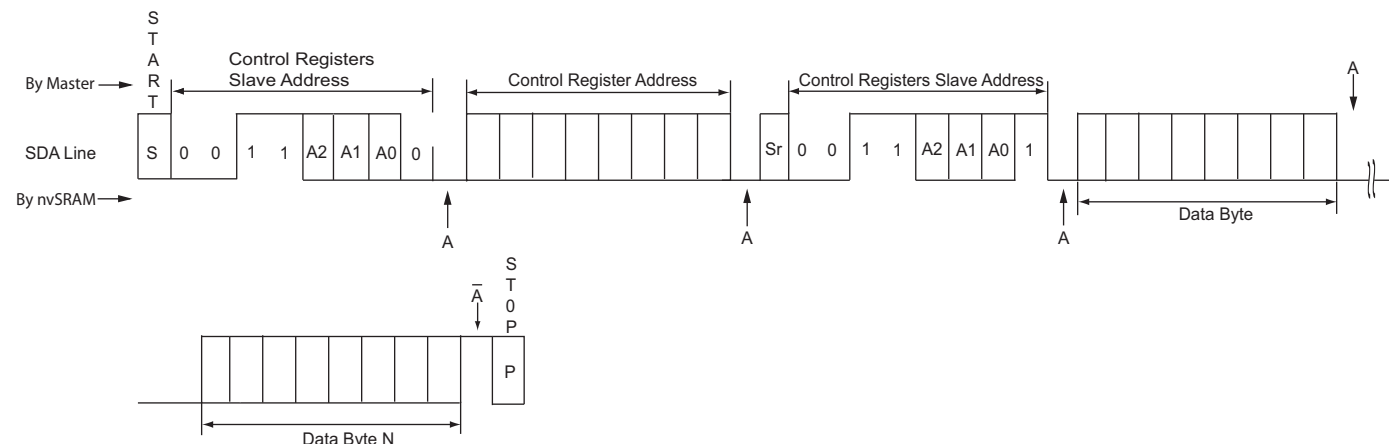
Figure 27. Random Control Registers Multi-Byte Read
