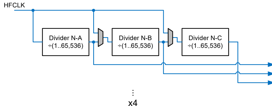
Figure 8-2. Peripheral Clock Divider Block Diagram
