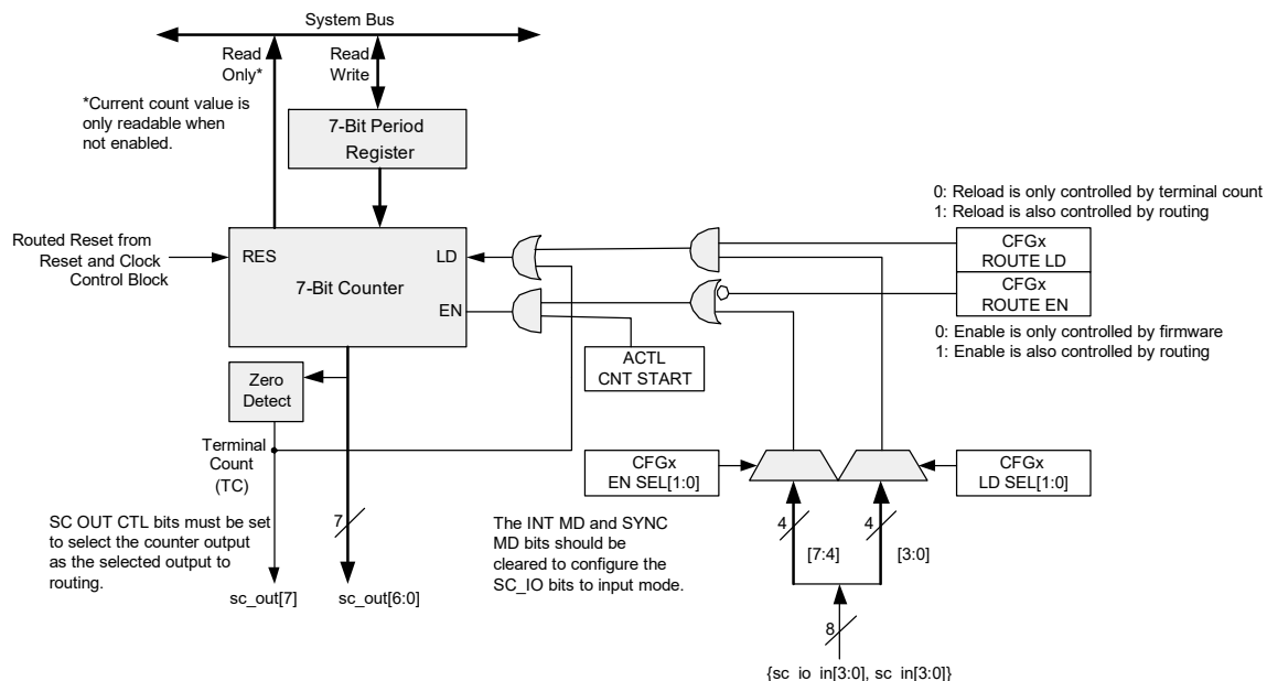
Figure 16-37. Counter Mode
