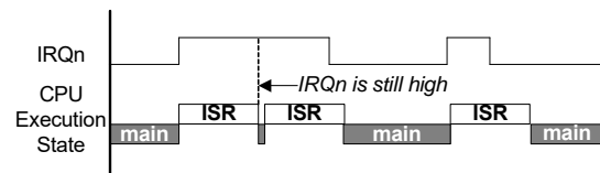
Figure 5-3. Level Interrupts
