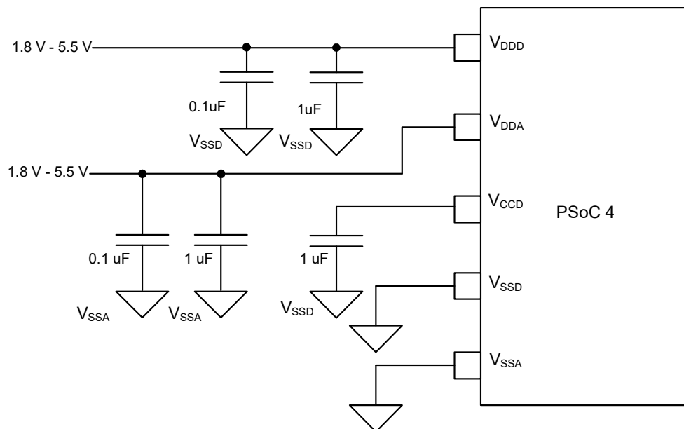
Figure 9-3. Separate Unregulated V DDA and V DD Supplies
