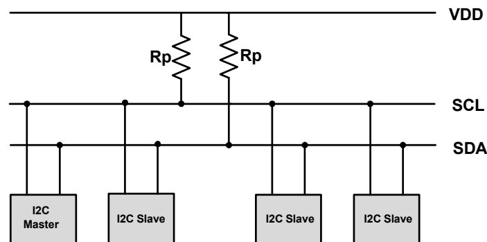
Figure 15-21. I 2 C Interface Block Diagram
