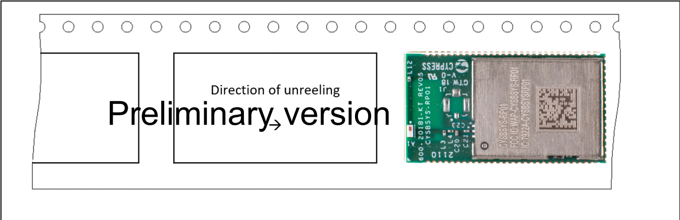
Figure 8 Tape dimensions
