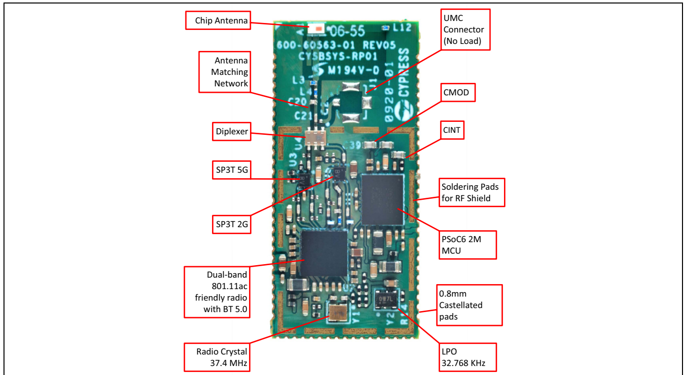
Figure 2 Key components
