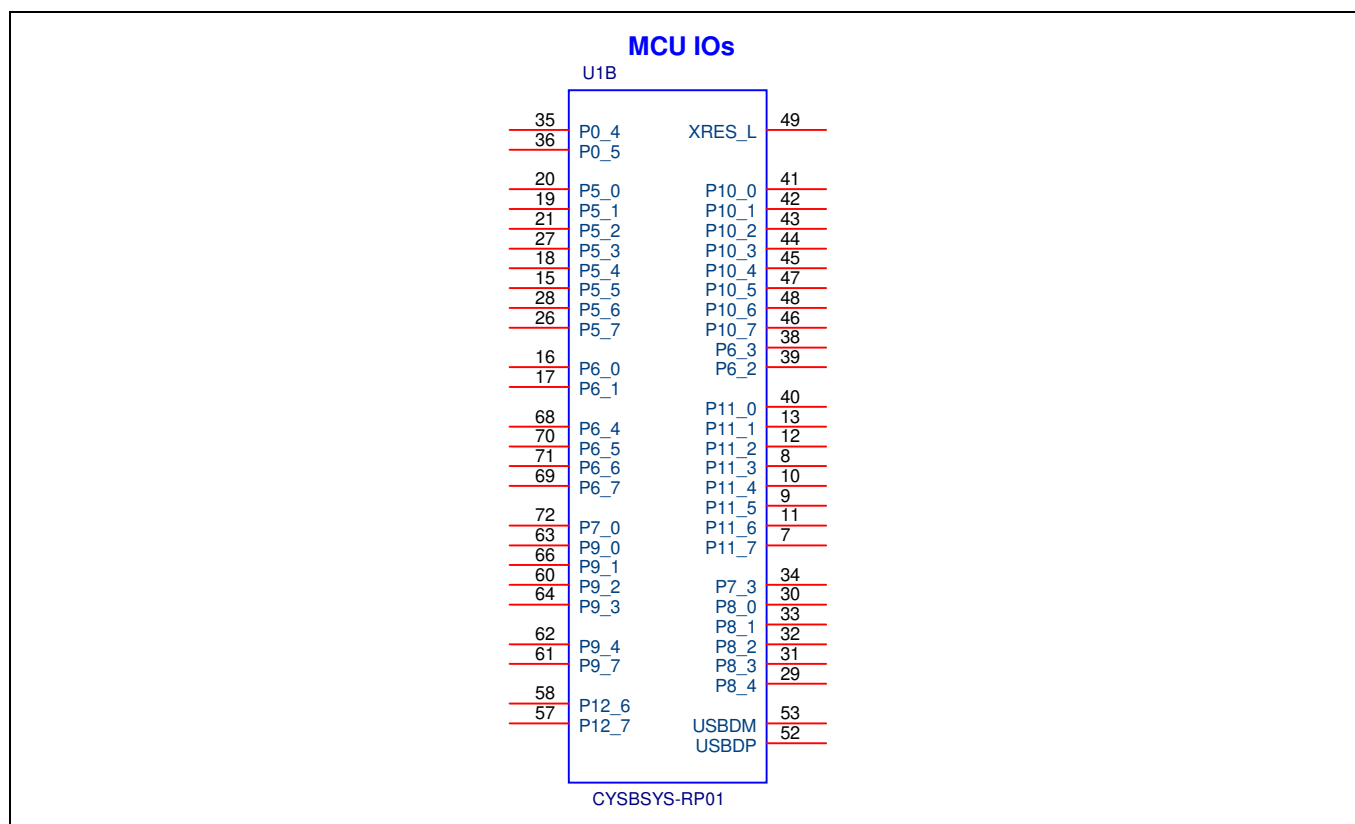
Figure 6 Castelled pads pinout
