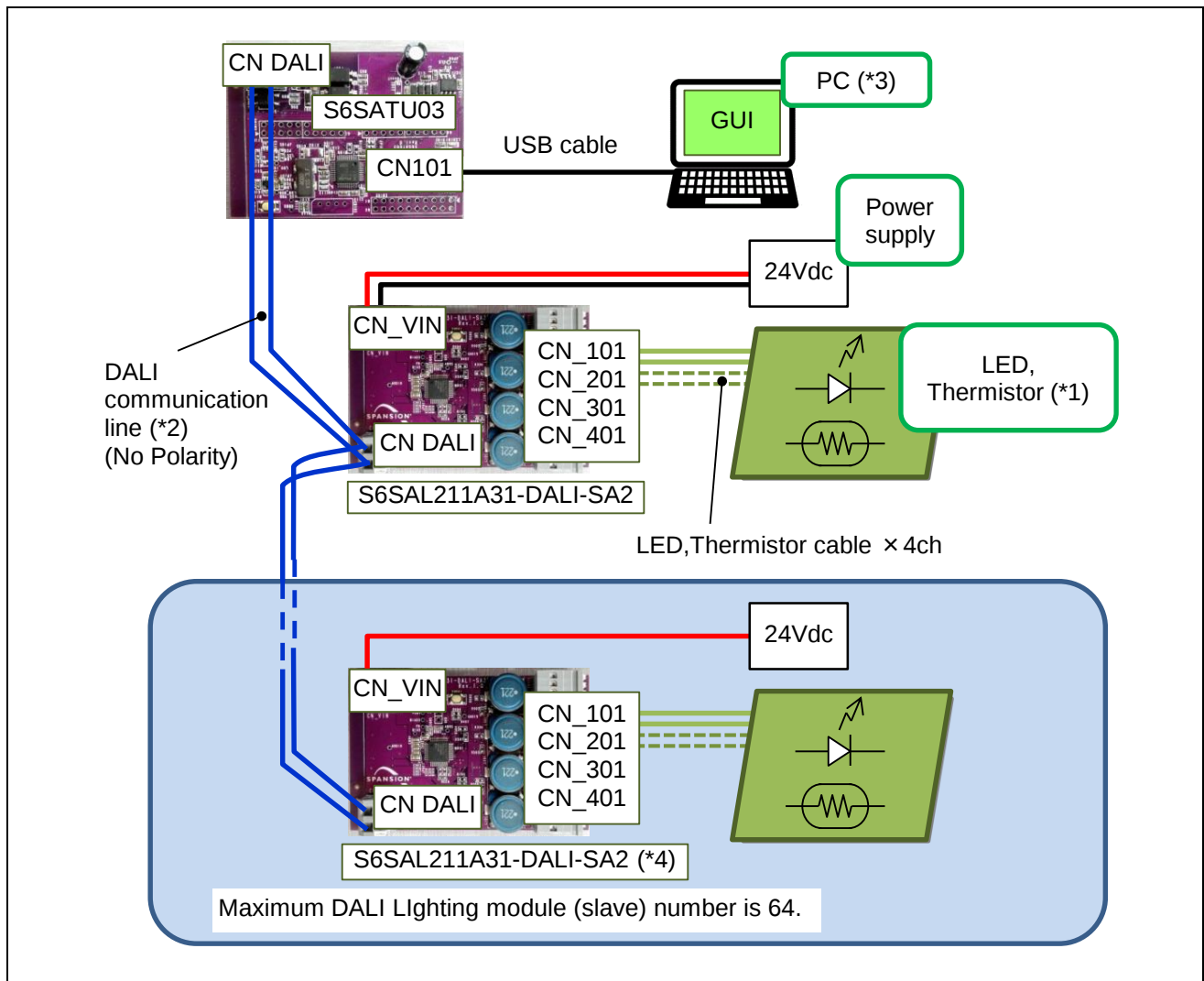
Figure 4-2 Board Connection
