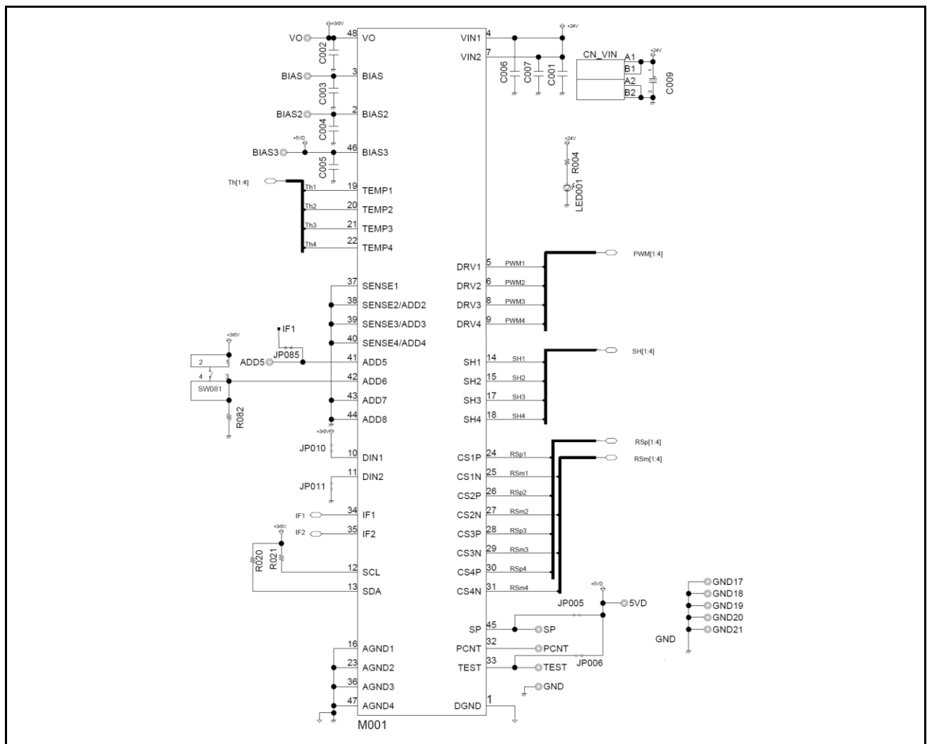
Figure 6-1 S6SAL211A31-DALI-SA2 Circuit Schematic
