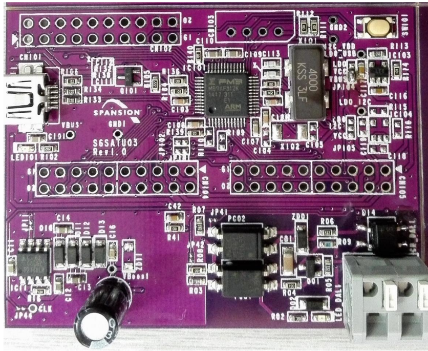
S6SATU03 (Top View)
