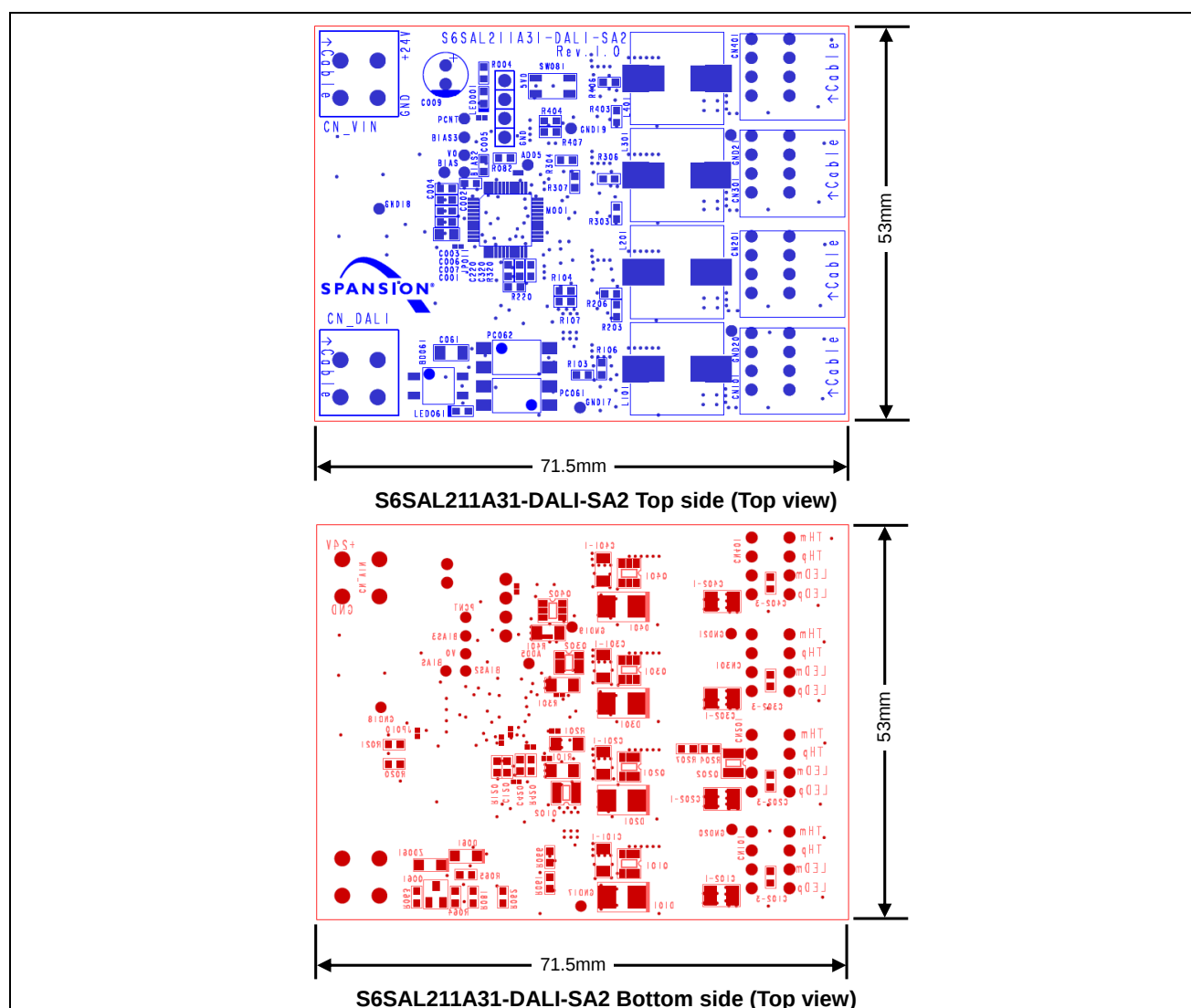
Figure 5-1 S6SAL211A31-DALI-SA2 Component Layout
