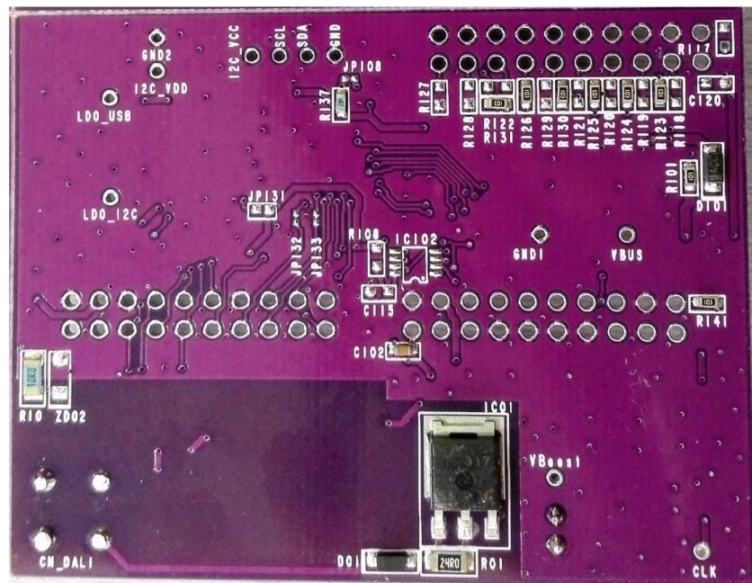
S6SATU03 (Bottom View)
