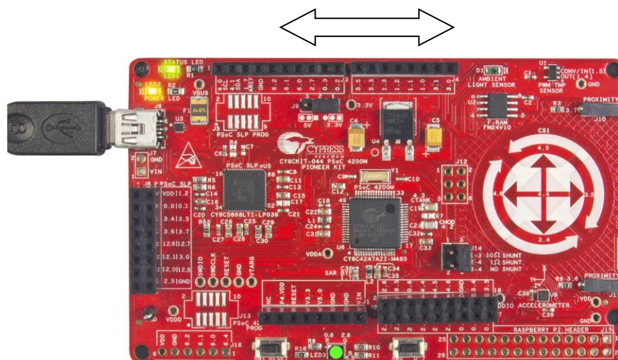
Figure 4-13 Accelerometer Movement in Y-Axis
