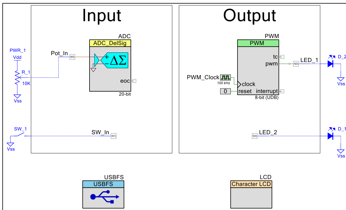
Figure 14. PSoC Creator Project Schematic Layout
