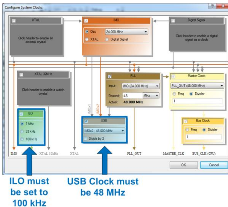
Figure 27. PSoC Clock Configuration
