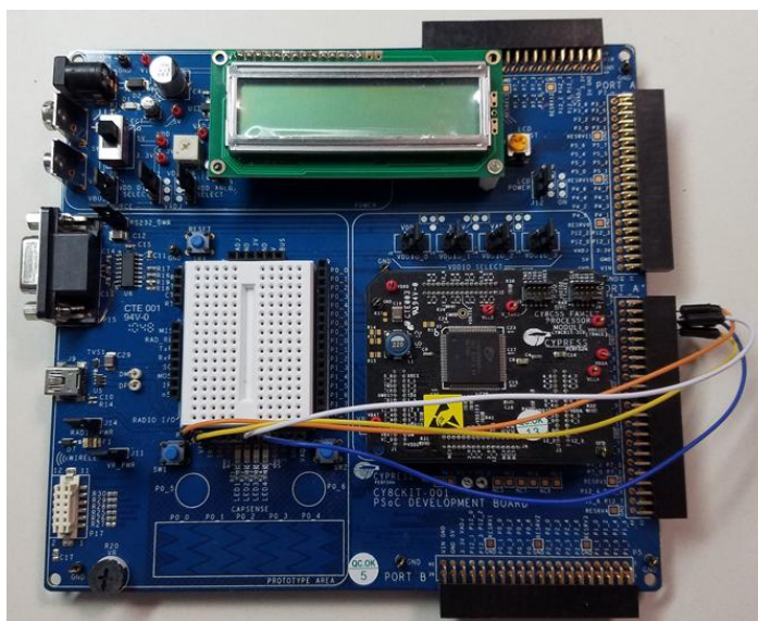
Figure 31. CY8CKIT-001 Configuration
