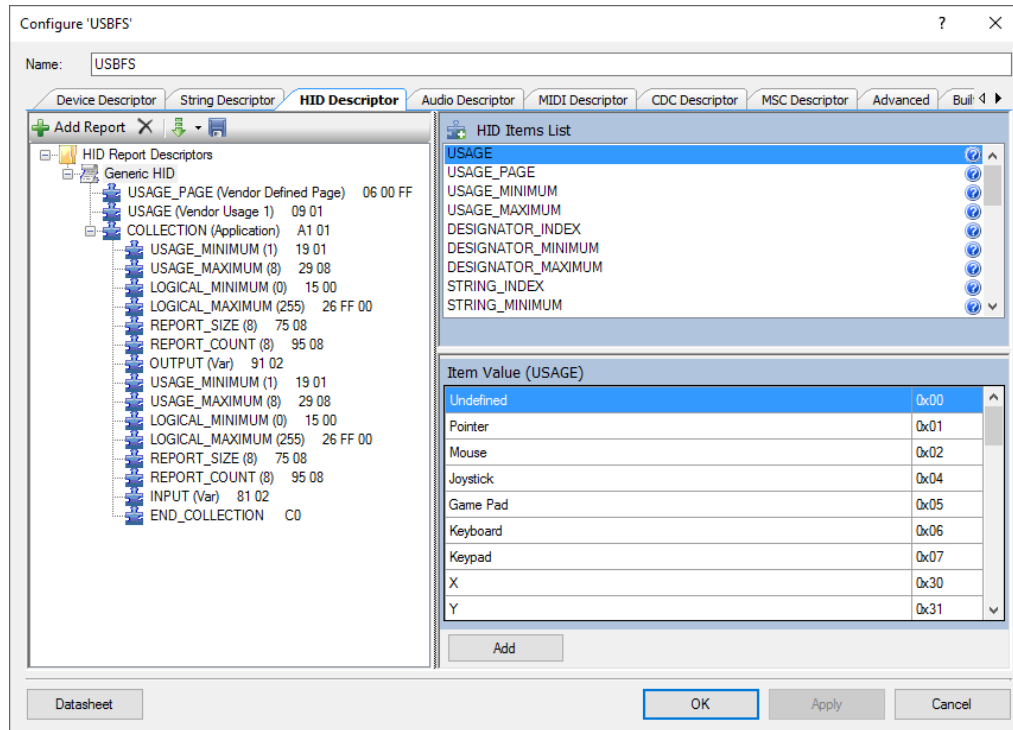
Figure 20. USBFS Completed HID Descriptor
