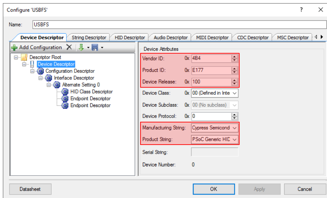
Figure 15. USBFS Device Descriptor Configuration
