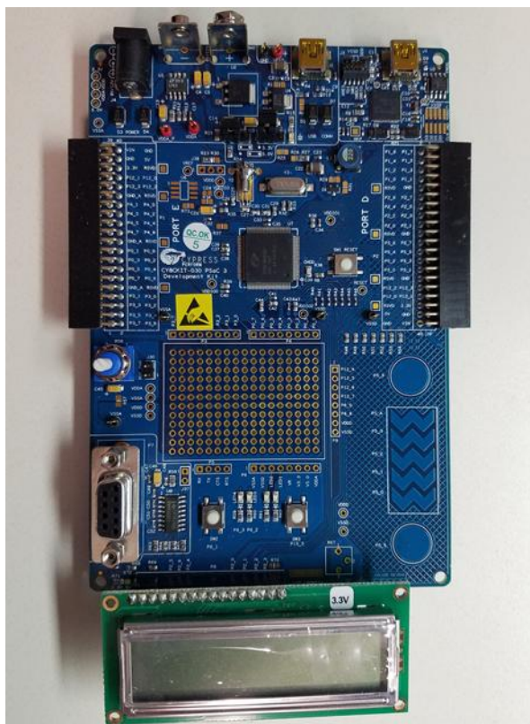
Figure 28. CY8CKIT-030/050 Configuration
