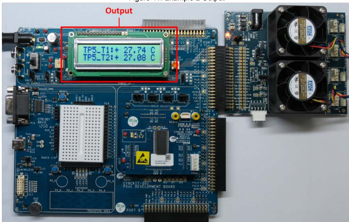
Figure 41. Example 2 Output
