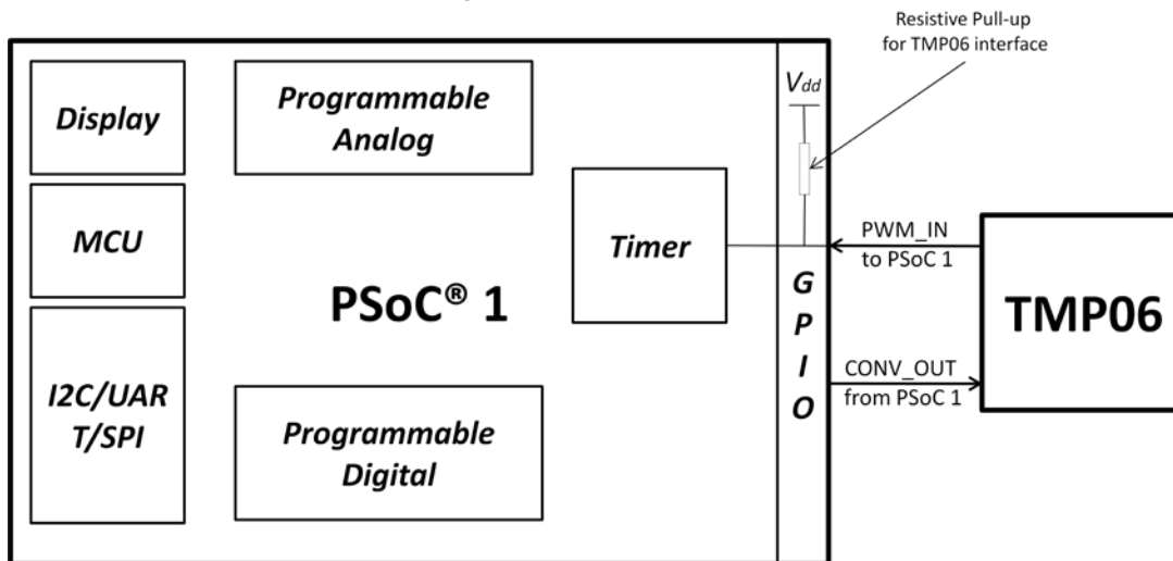
Figure 2. PSoC with TMP06
