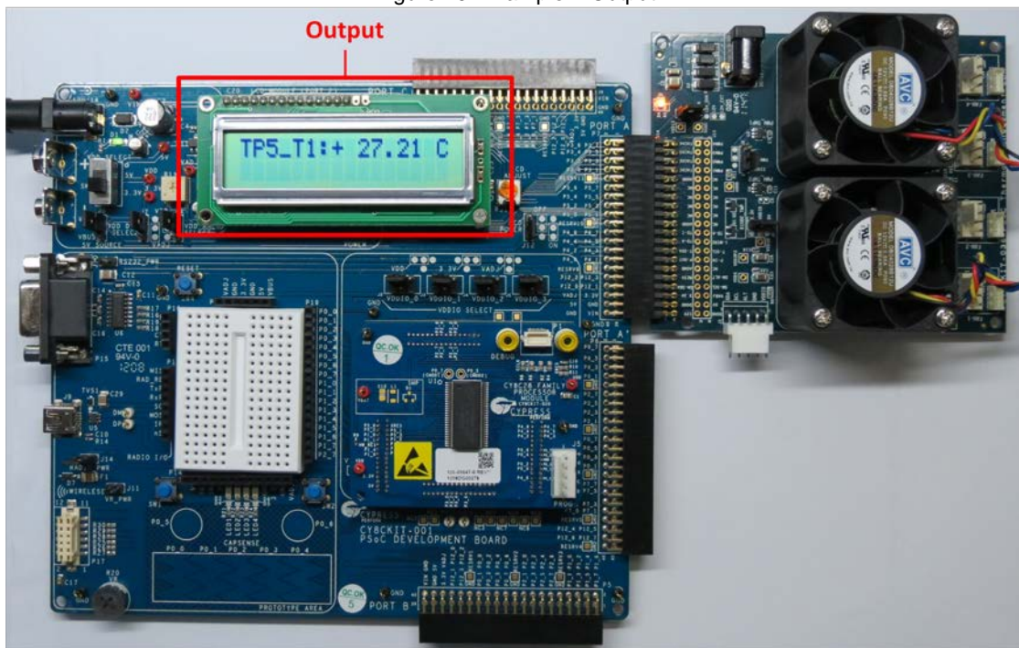
Figure 40. Example 1 Output
