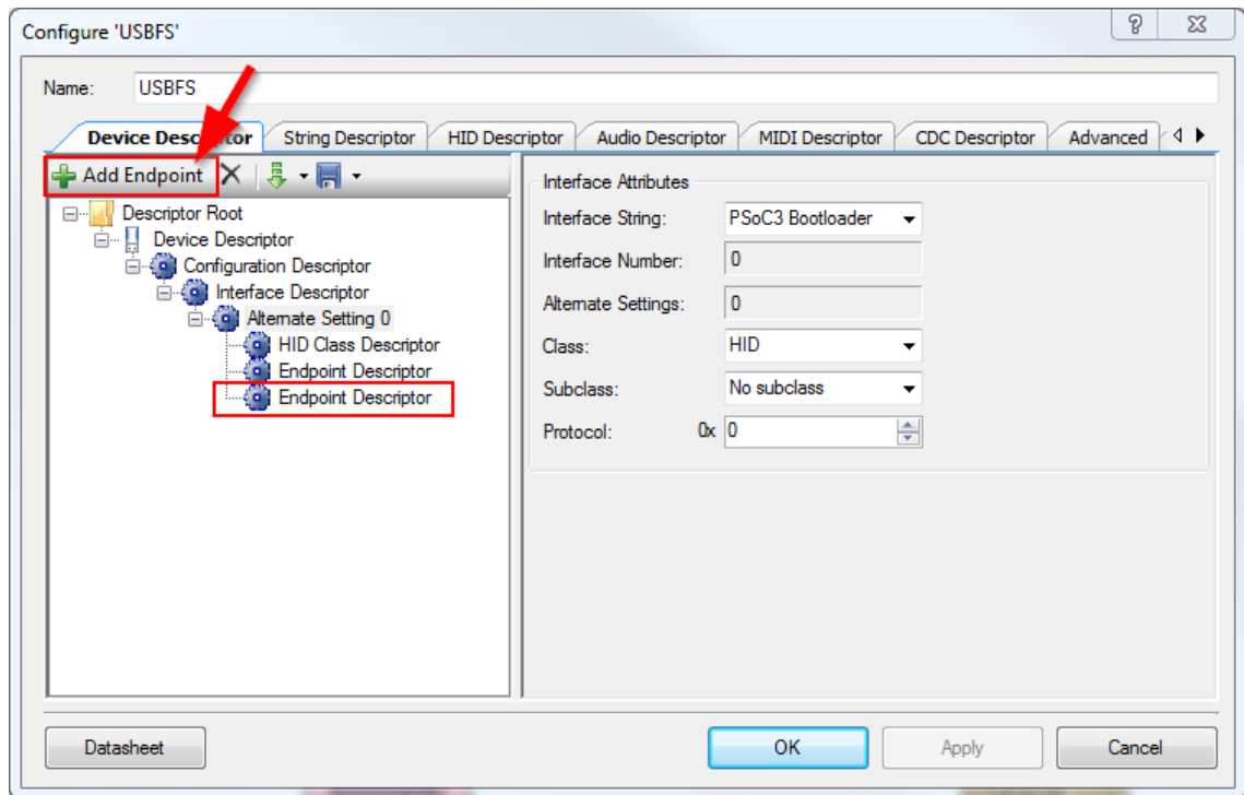
Figure 20. USBFS Adding Endpoints
