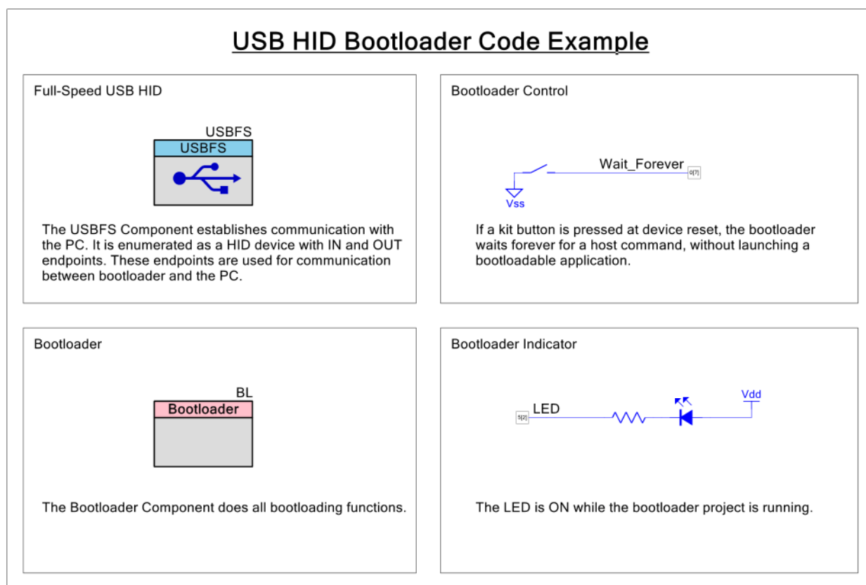
Figure 3. Bootloader Project Schematic from Code Example CE95391
