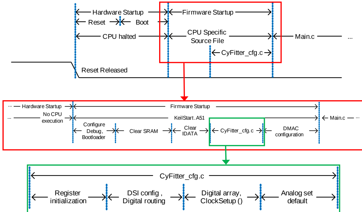
Figure 26. Device Startup Process Diagrams
