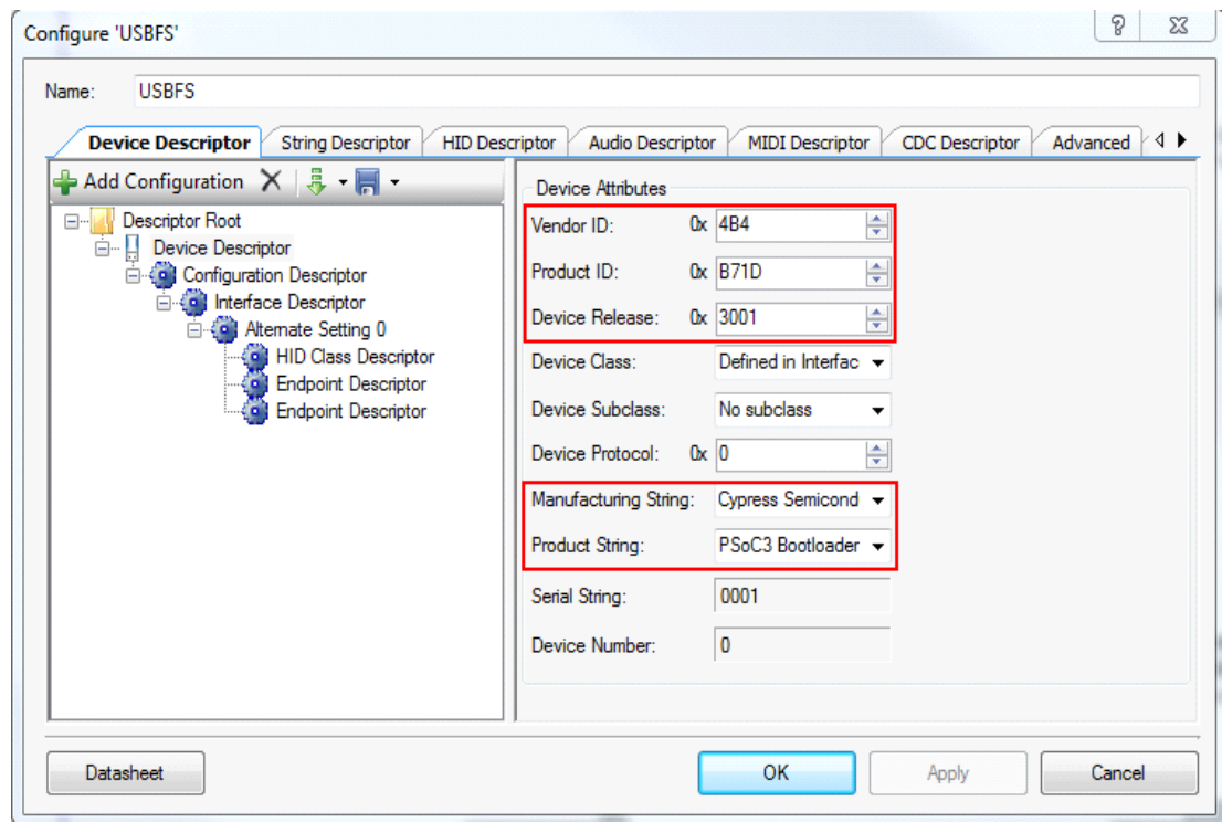
Figure 16. USBFS Device Descriptor
