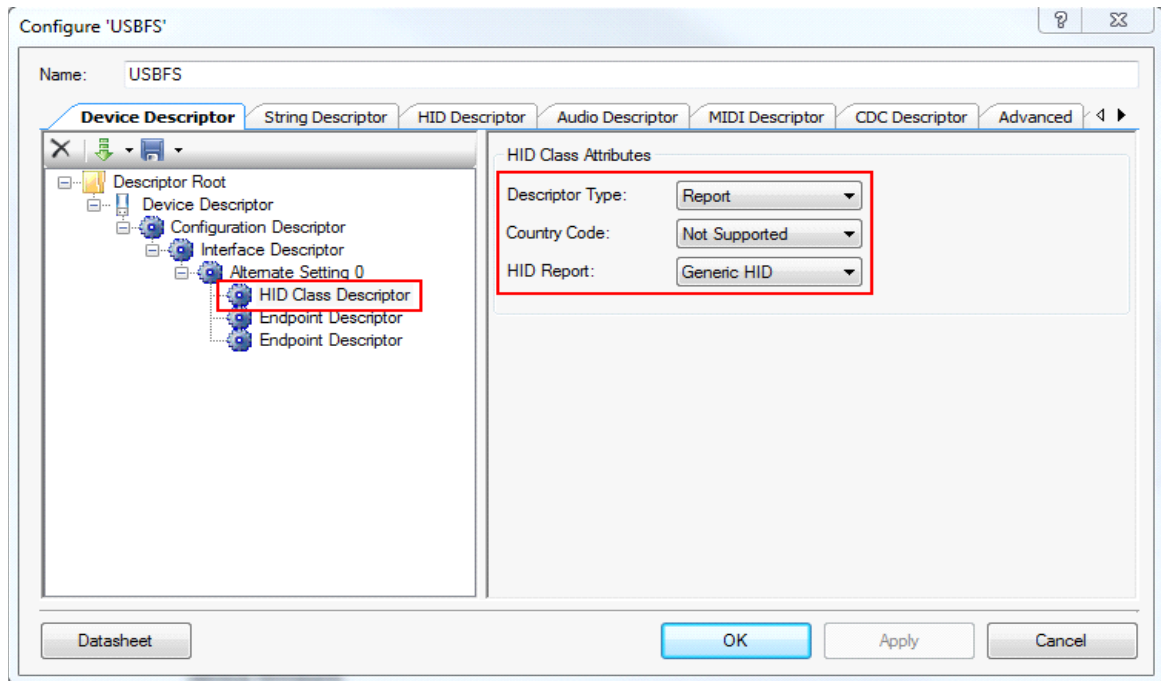
Figure 23. USBFS HID Device Attributes
