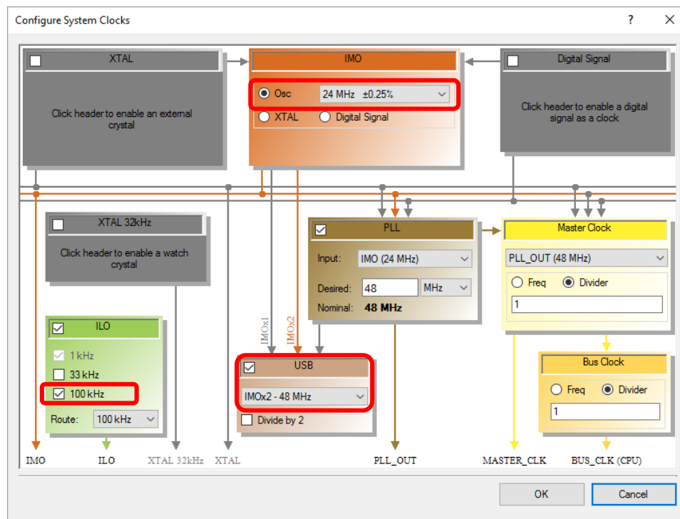
Figure 8. PSoC 3 and PSoC 5LP USB Clock Configuration
