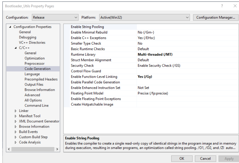
Figure 14. Runtime Library Option
