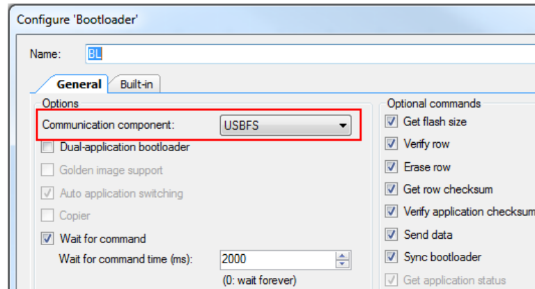
Figure 4. Bootloader Component Customizer
