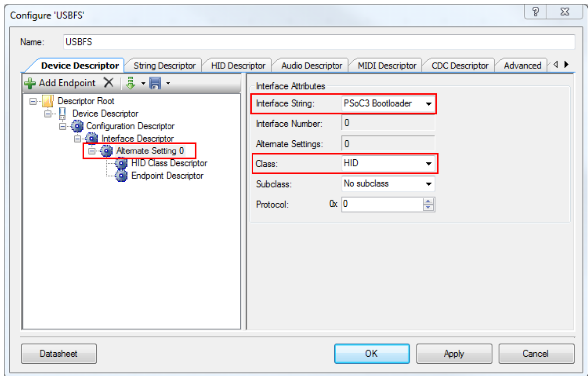
Figure 19. USBFS Alternate Setting
