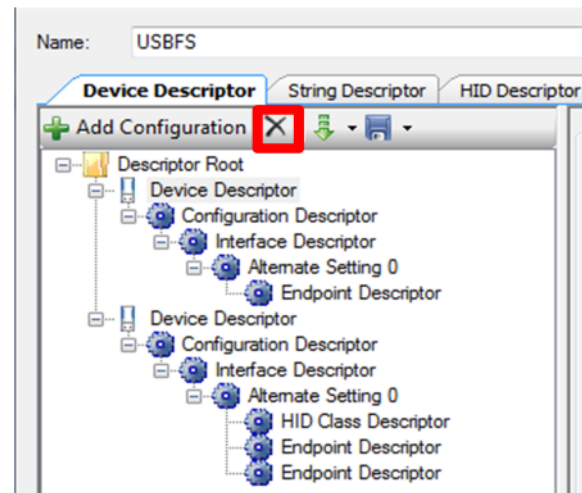
Figure 5. Delete Default USB Configuration
