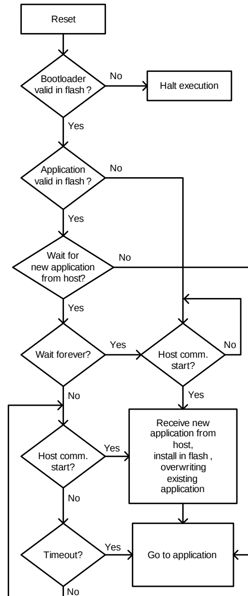
Figure 2. Bootload Process Flowchart
