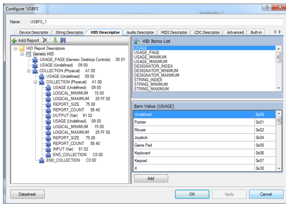
Figure 22. Completed HID Descriptor
