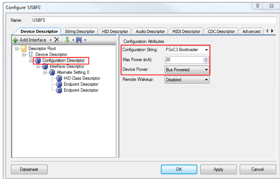
Figure 18. USBFS Configuration Descriptor
