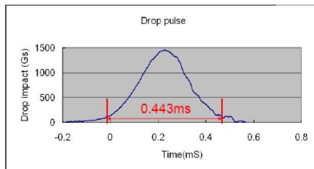
Figure 21. Drop Test Impact Force Profile
