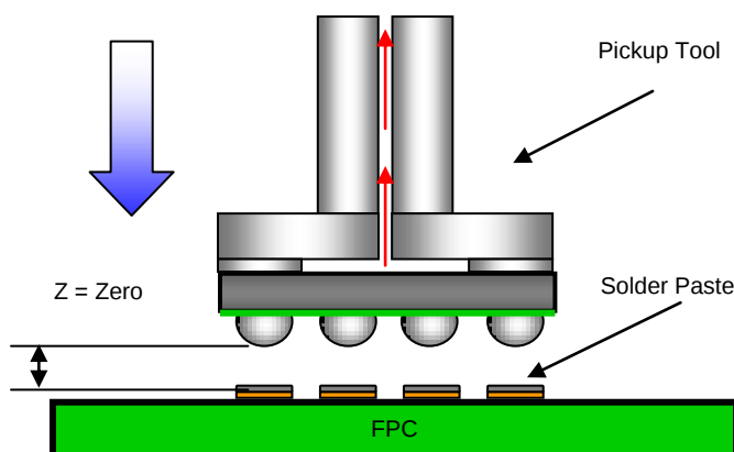
Figure 11. WLCSP Placement on FPC Board
