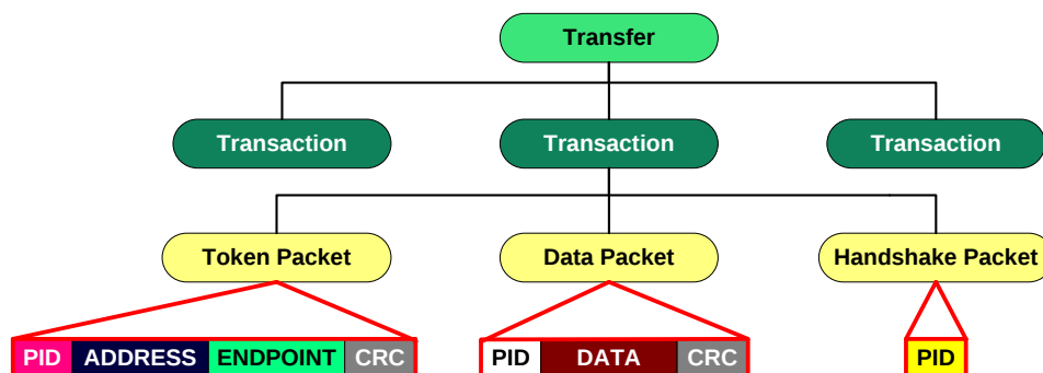
Figure 1. Structure of a USB Transfer
