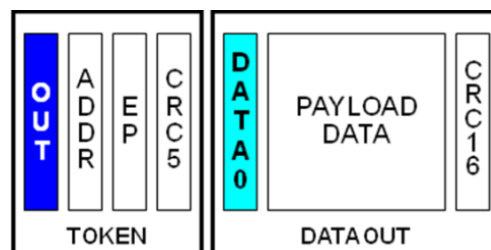
Figure 20. Example of an OUT Isochronous Transaction
