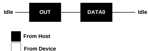
Figure 18. Flowchart of an OUT Isochronous Transaction
