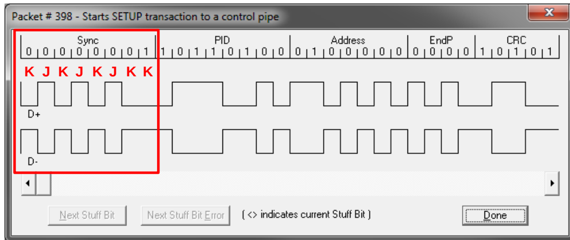
Figure 3. Full Speed SYNC Field
