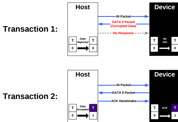
Figure 39. Example of Data Toggle with Corrupted Data
