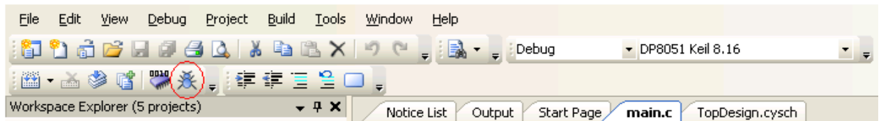
Figure 25. Debug Button
