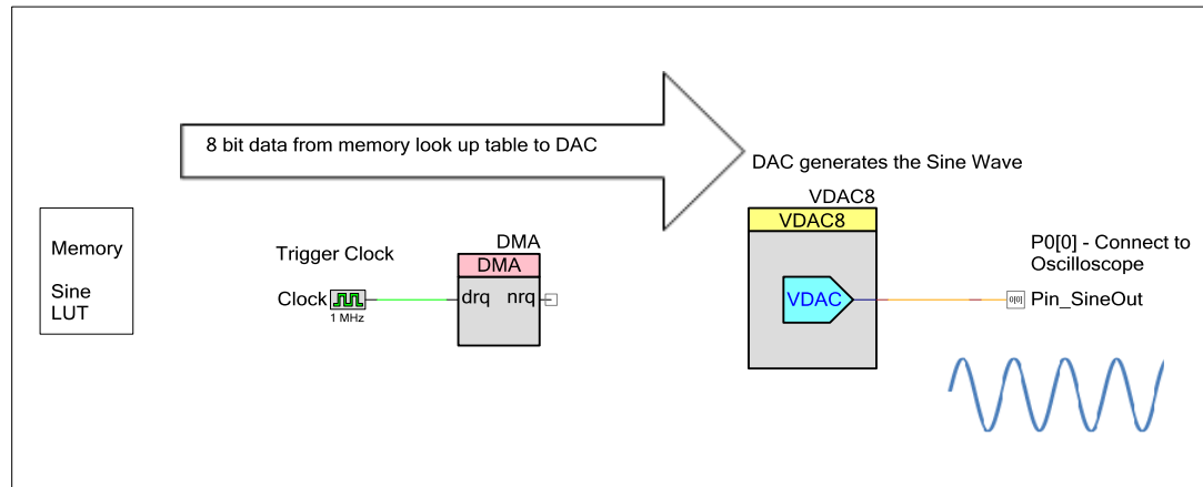
Figure 11. Top Design, Memory-to-Peripheral Transfer
