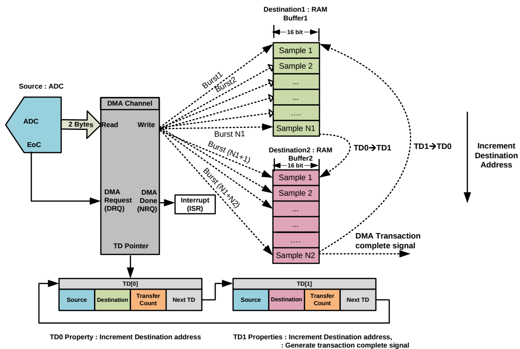
Figure 14. Block Diagram, TD Chaining
