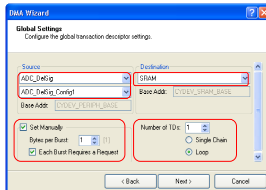
Figure 16. Global Settings
