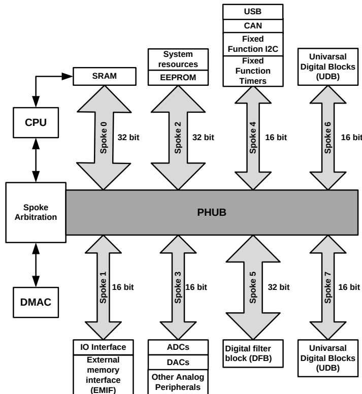
Figure 1. Peripheral HUB
