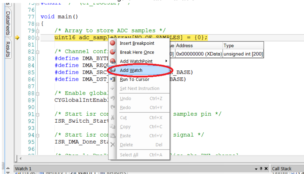
Figure 21. Watch Variable
