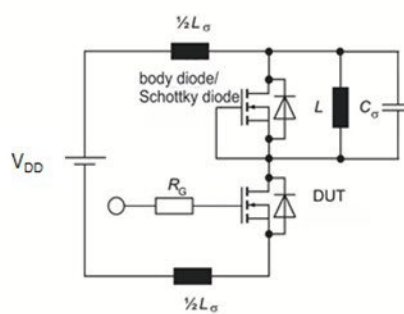
Figure E. Dynamic test circuit
