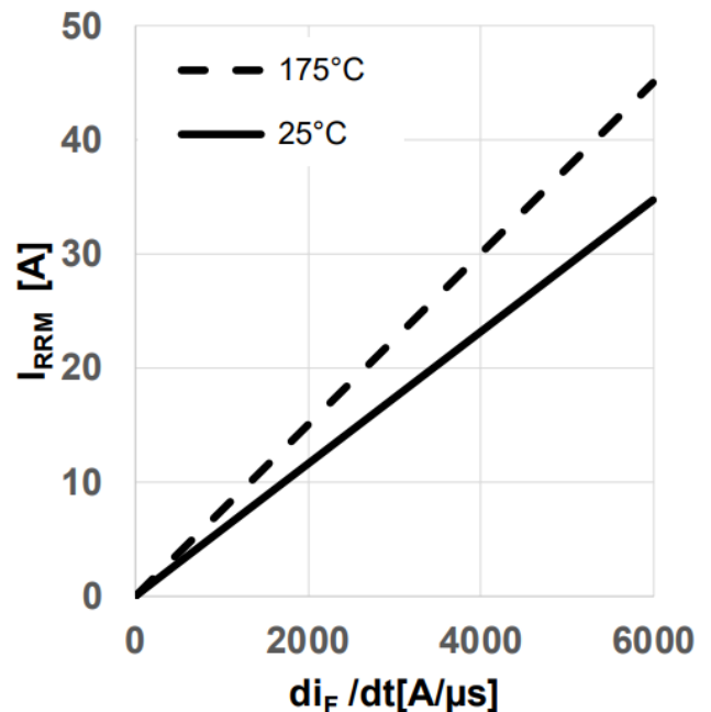
Figure 20 Typical reverse recovery current as a function of diode current slope (I_{rrm} = f(di_F/dt), V_{DD} = 800V, V_{GS} = 0V/18V, I_D = 25A, \text{ind. load, test circuit in Fig. E,} body diode at V_{GS} = 0V )
