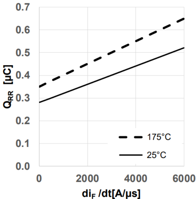
Figure 19 Typical reverse recovery charge as a function of diode current slope (Q_{rr} = f(di_F/dt), V_{DD} = 800V, V_{GS} = 0V/18V, I_D = 25A, \text{ind. load, test circuit in Fig. E,} body diode at V_{GS} = 0V )
