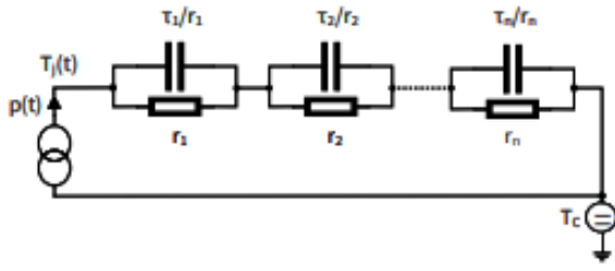
Figure E. Thermal equivalent circuit
