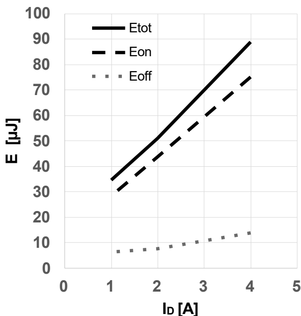
图 16 典型开关能量损耗随漏源电流变化关系 ( E = f(I_{DS}) , V_{DD} = 800\text{V} , V_{GS} = 0\text{V}/18\text{V} , R_{G,ext} = 2\Omega , T_{vj} = 175^{\circ}\text{C} , ind. load, test circuit in Fig. E, diode: body diode at V_{GS} = 0\text{V} )
