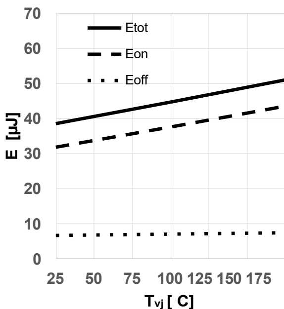
图 15 典型开关能量损耗随结温变化关系 ( E = f(T_{vj}) , V_{DD} = 800\text{V} , V_{GS} = 0\text{V}/18\text{V} , R_{G,ext} = 2\Omega , I_D = 2\text{A} , ind. load, test circuit in Fig. E, diode: body diode at V_{GS} = 0\text{V} )
