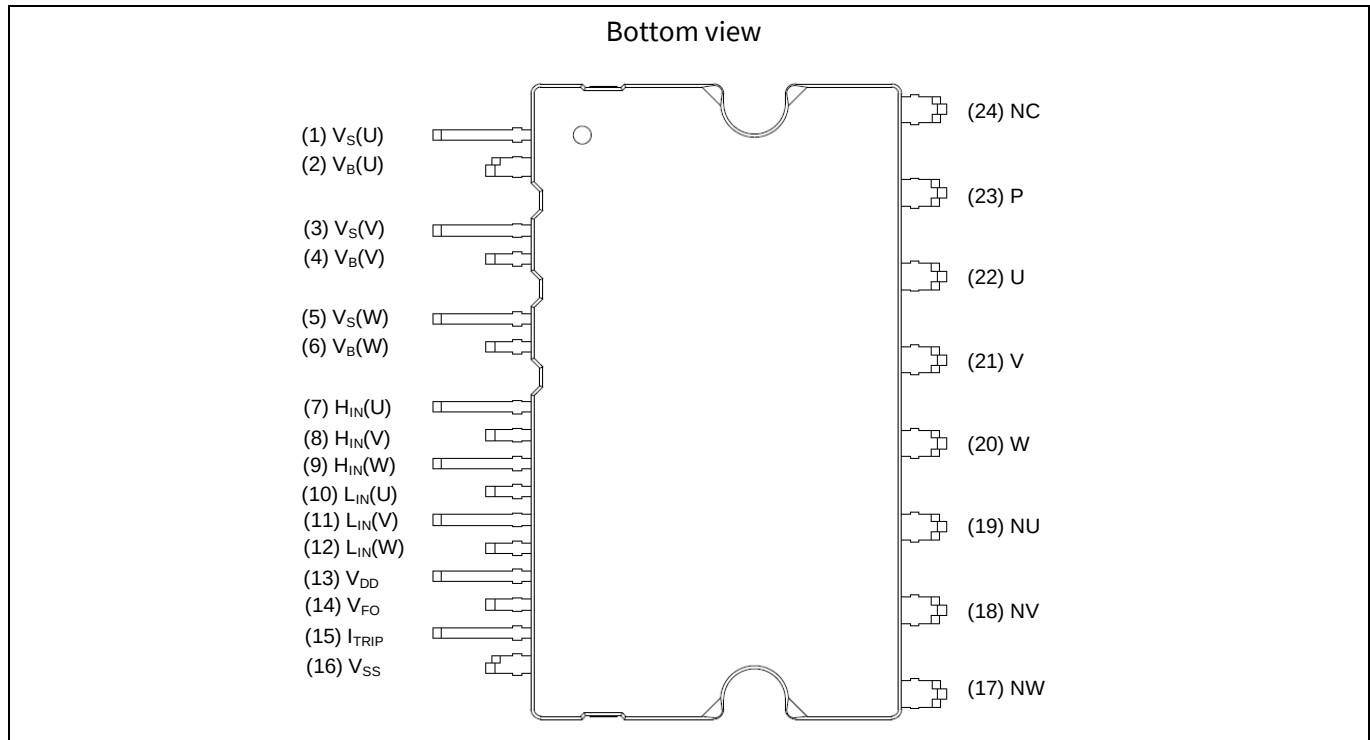
Figure 2 Pin configuration
