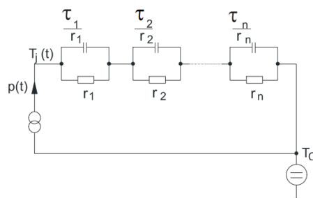
Figure D. Thermal equivalent circuit
