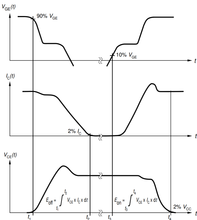
Figure B. Definition of switching losses
