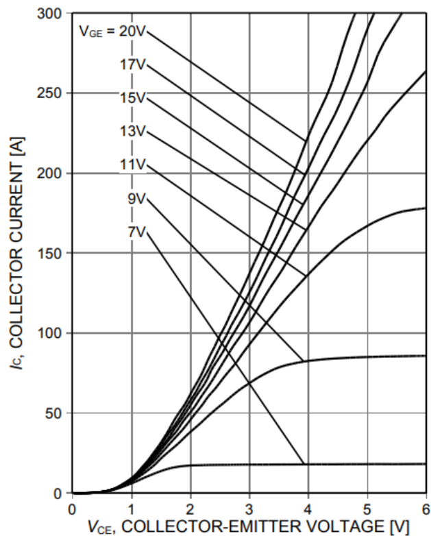
Figure 3. Typical output characteristic ( T_{vj}=175^{\circ}\text{C} )
