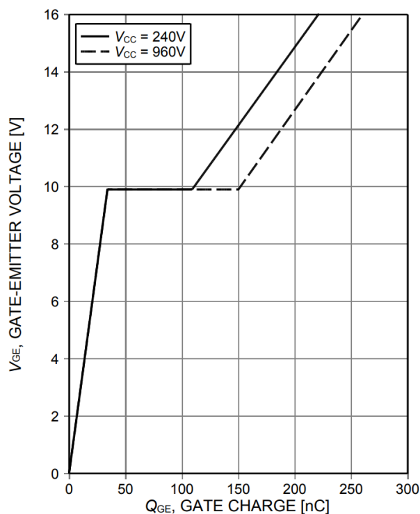
Figure 16. Typical gate charge ( I_C=50\text{A} )
