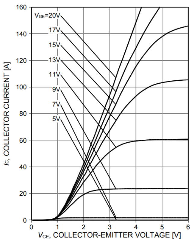
Figure 4. Typical output characteristic ( T_{vj}=25^\circ\text{C} )
