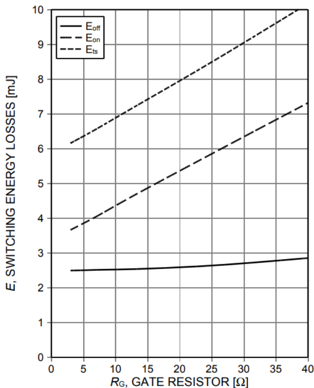
Figure 13. Typical switching energy losses as a function of gate resistor (inductive load, T_{vj}=175^\circ\text{C} , V_{CE}=600\text{V} , V_{GE}=0/15\text{V} , I_C=40\text{A} , Dynamic test circuit in Figure E)
