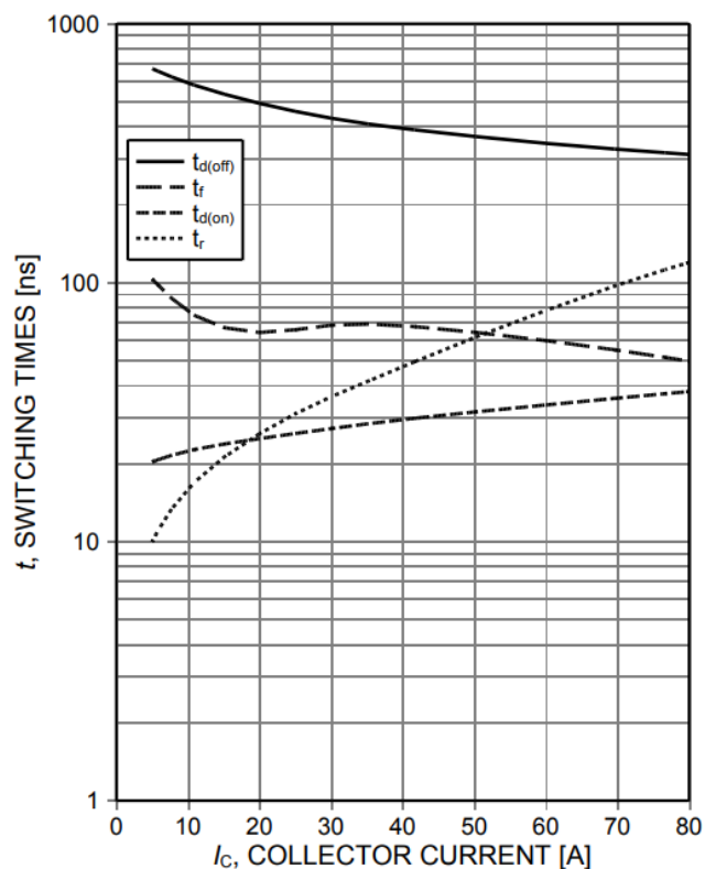
Figure 8. Typical switching times as a function of collector current (inductive load, T_{vj}=175^{\circ}\text{C} , V_{ce}=600\text{V} , V_{ge}=0/15\text{V} , R_G=12\Omega , Dynamic test circuit in
