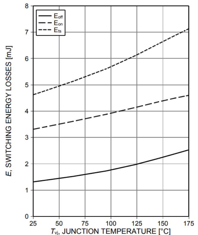
Figure 14. Typical switching energy losses as a function of junction temperature (inductive load, V_{CE}=600\text{V} , V_{GE}=0/15\text{V} , I_C=40\text{A} , R_G=12\Omega , Dynamic test circuit in Figure E)
