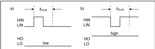
Figure 4 Input filter timing diagram
