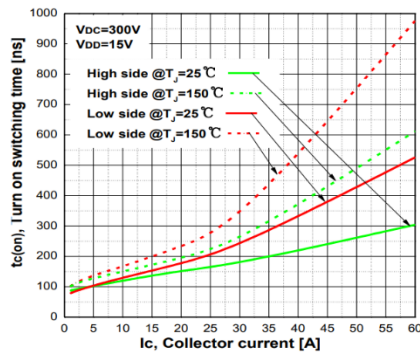
Typ. Turn on switching time
