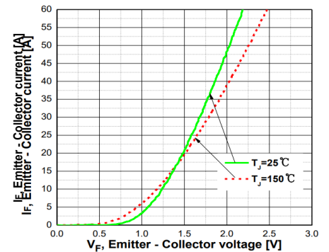
Typ. Diode forward voltage
