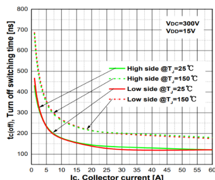
Typ. Turn off switching time
