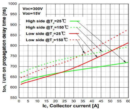
Typ. Turn on propagation delay time
