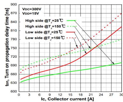
Typ. Turn on propagation delay time
