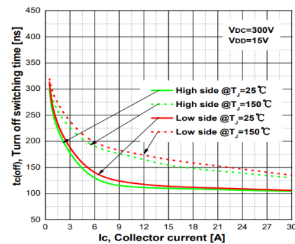
Typ. Turn off switching time
