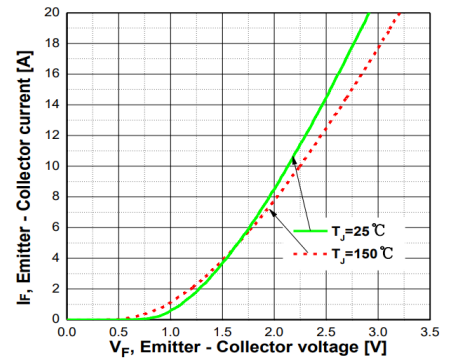
Typ. Diode forward voltage
