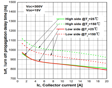
Typ. Turn off propagation delay time
