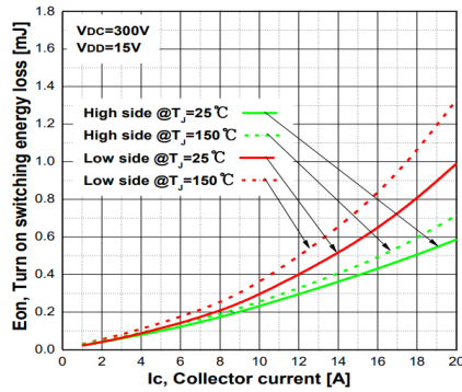
Typ. Turn on switching energy loss
