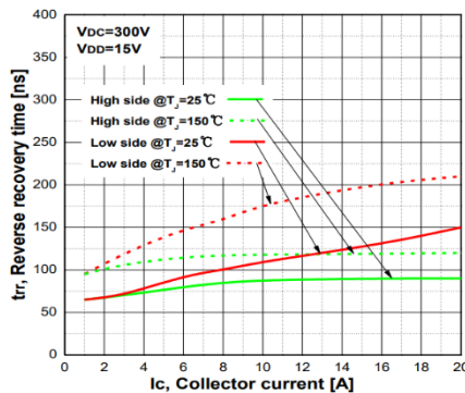
Typ. Reverse recovery time
