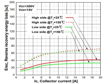
Typ. Reverse recovery energy loss
