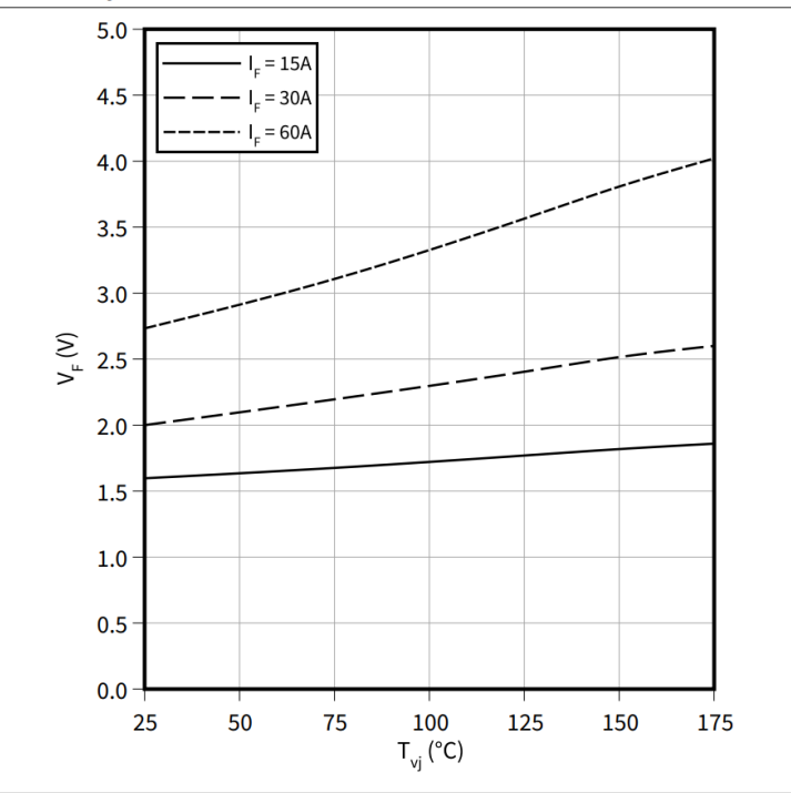
Typical diode forward voltage as a function of junction temperature V_F = f(T_{vj})
