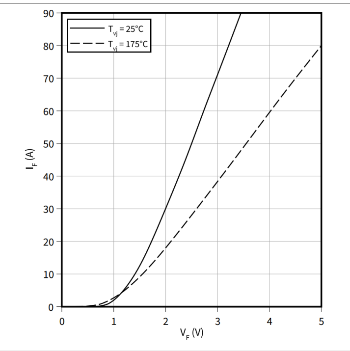
Typical diode forward current as a function of forward voltage I_F = f(V_F)
