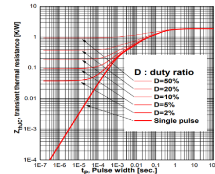
IGBT transient thermal resistance at all IGBTs operation
