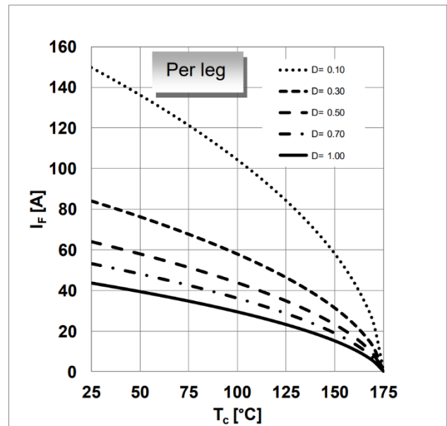
Figure 2. Diode forward current per leg as function of temperature , parameter: T_j \leq 175^\circ\text{C} , R_{\text{th(j-c),max}} , D =duty cycle, V_{\text{th}} , R_{\text{diff}} @ T_j=175^\circ\text{C}
