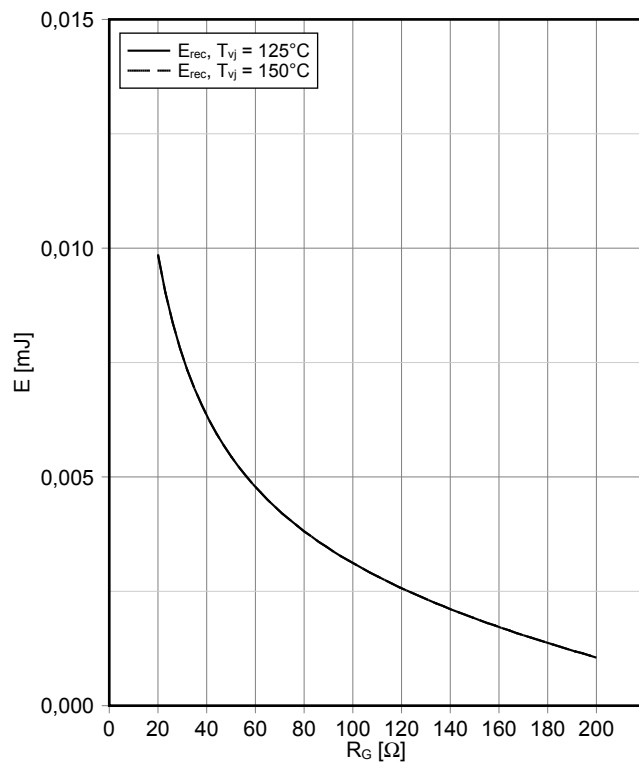
开关损耗 二极管, 三电平 (典型) switching losses Diode, 3-Level (typical) E_{rec} = f(R_G) I_F = 10\ \text{A} , V_{CE} = 300\ \text{V}
