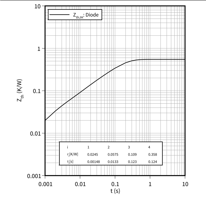
瞬态热阻抗, 反极性保护二极管 A Z_{th} = f(t)
