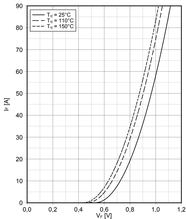
順方向特性 逆極性保護 diode A ( 典型) forward characteristic of Inverse-polarity protection diode A (typical) I_F = f(V_F)
