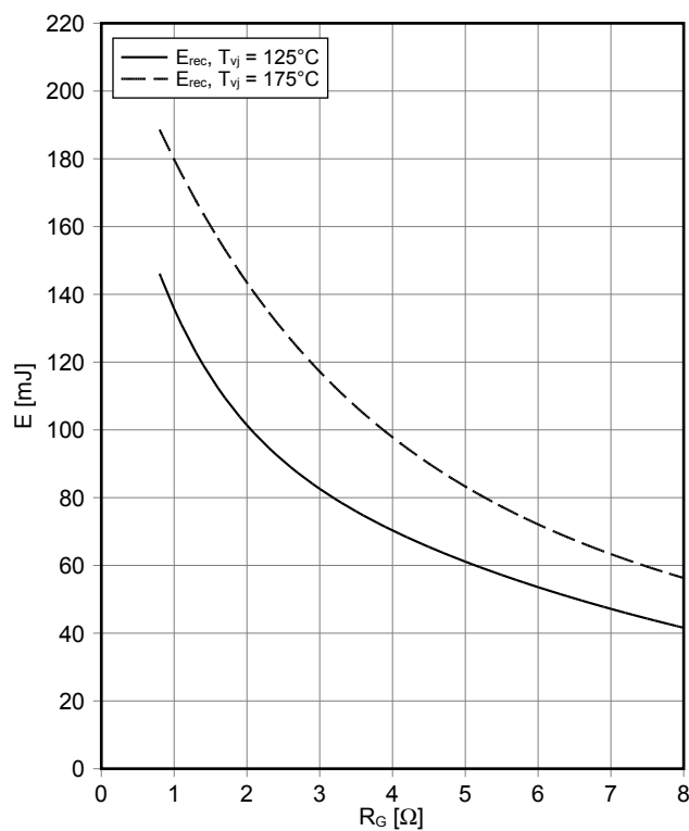
开关损耗 二极管,逆变器 (典型) switching losses Diode, Inverter (typical) E_{rec} = f(R_G) I_F = 1800 \text{ A} , V_{CE} = 600 \text{ V}
