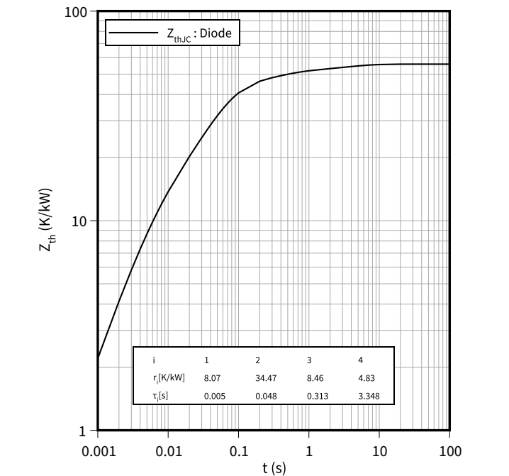
瞬态热阻抗，二极管，制动-斩波器 Z_{th} = f(t)
