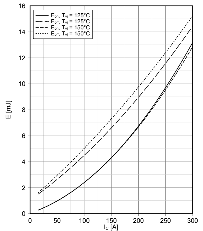
スイッチング損失 IGBT, T1 / T4 (Typical) switching losses IGBT, T1 / T4 (typical) E_{on} = f(I_C) , E_{off} = f(I_C) V_{GE} = \pm 15\text{ V} , R_{Gon} = 5\ \Omega , R_{Goff} = 20\ \Omega , V_{CE} = 500\text{ V}
