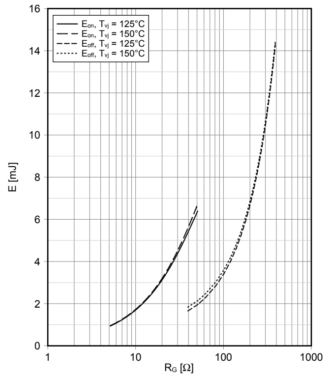
开关损耗 IGBT, T2 / T3 (典型) switching losses IGBT, T2 / T3 (typical)
