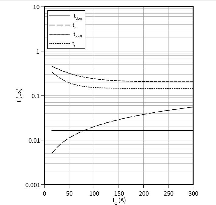
スイッチング時間 (typical), IGBT, T2 / T3 t = f(IC) RGoff = 1.5 Ω, RGon = 1.5 Ω, VGE = ±15 V, VCE = 300 V, TVj = 150 °C
