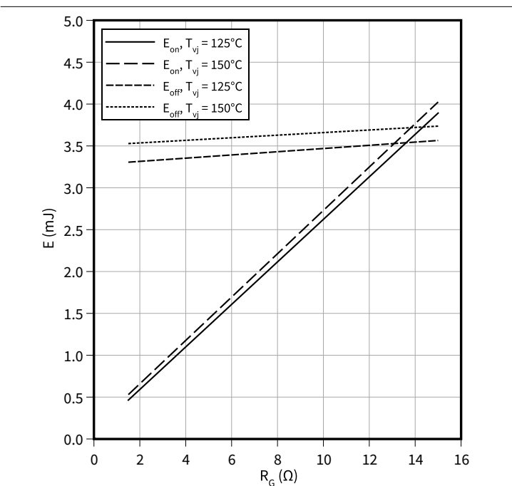
开关损耗 (典型), IGBT, T2 / T3 E = f(RG) VGE = ±15 V, IC = 100 A, VCE = 300 V
