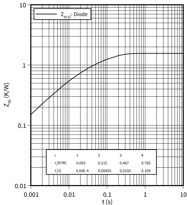
transient thermal impedance, Diode, Rectifier Z_{th} = f(t)
