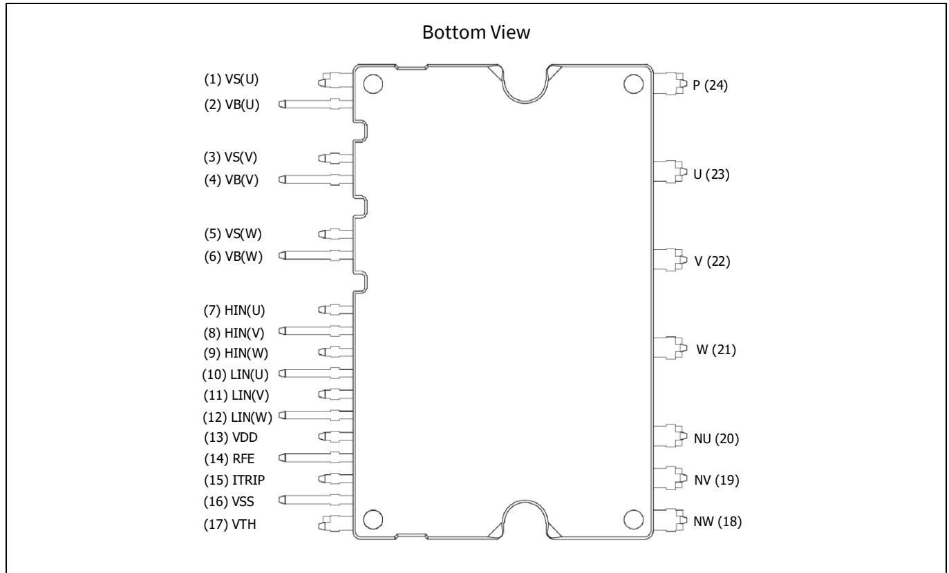
Figure 2 Module pinout
