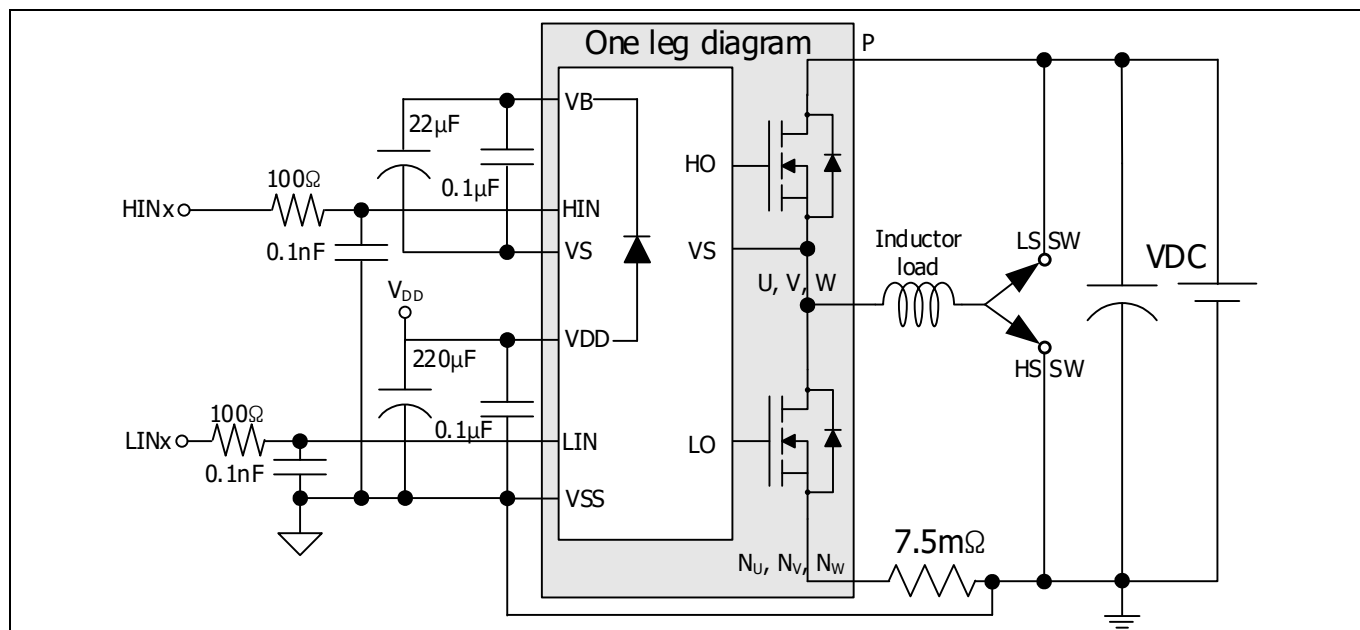
Figure 9 Switching test circuit
