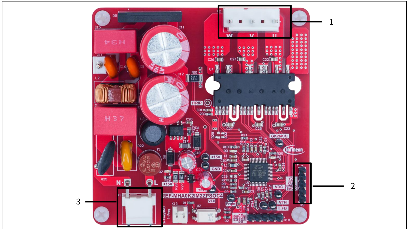
Figure 3 Connectors of the REF-MHA0K2IM2ZPSOC4 reference board
