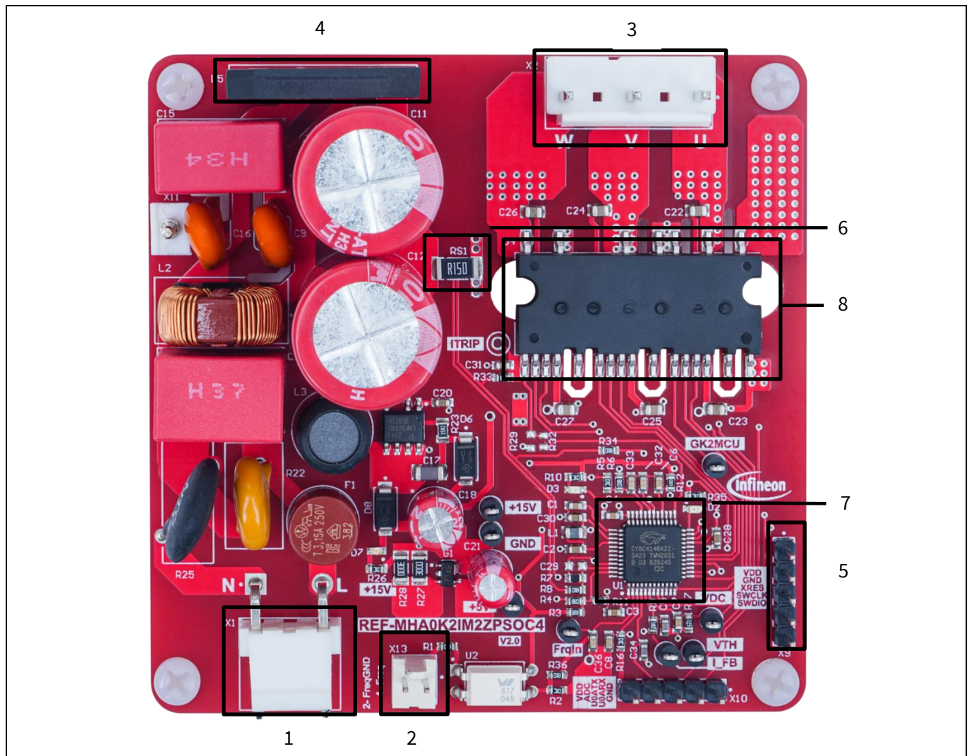
Figure 2 Functional groups of the REF-MHA0K2IM2ZPSOC4 reference board
