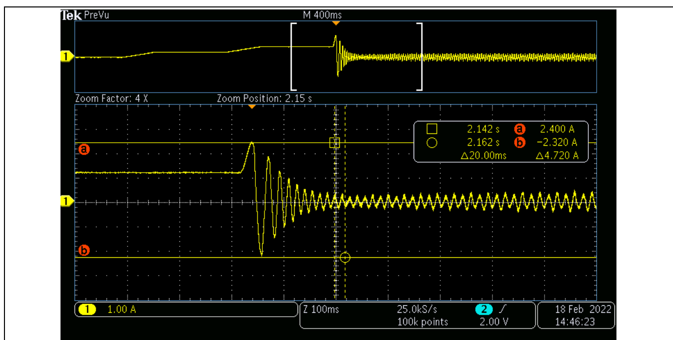
Figure 18 Start-up waveform of fridge at empty load
