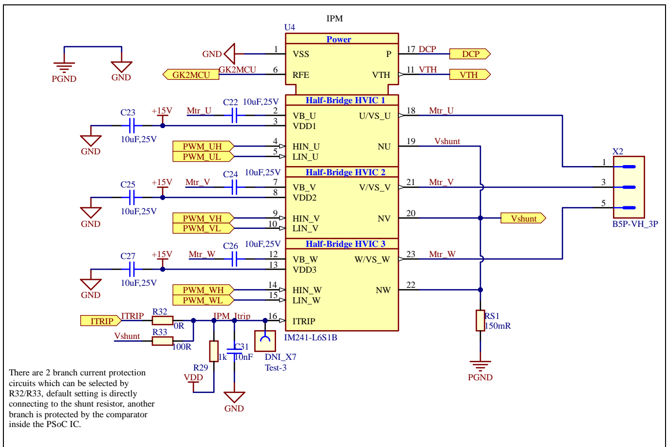
Figure 6 Schematic of inverter section using IM241-L6S1B CIPOS™ Micro
