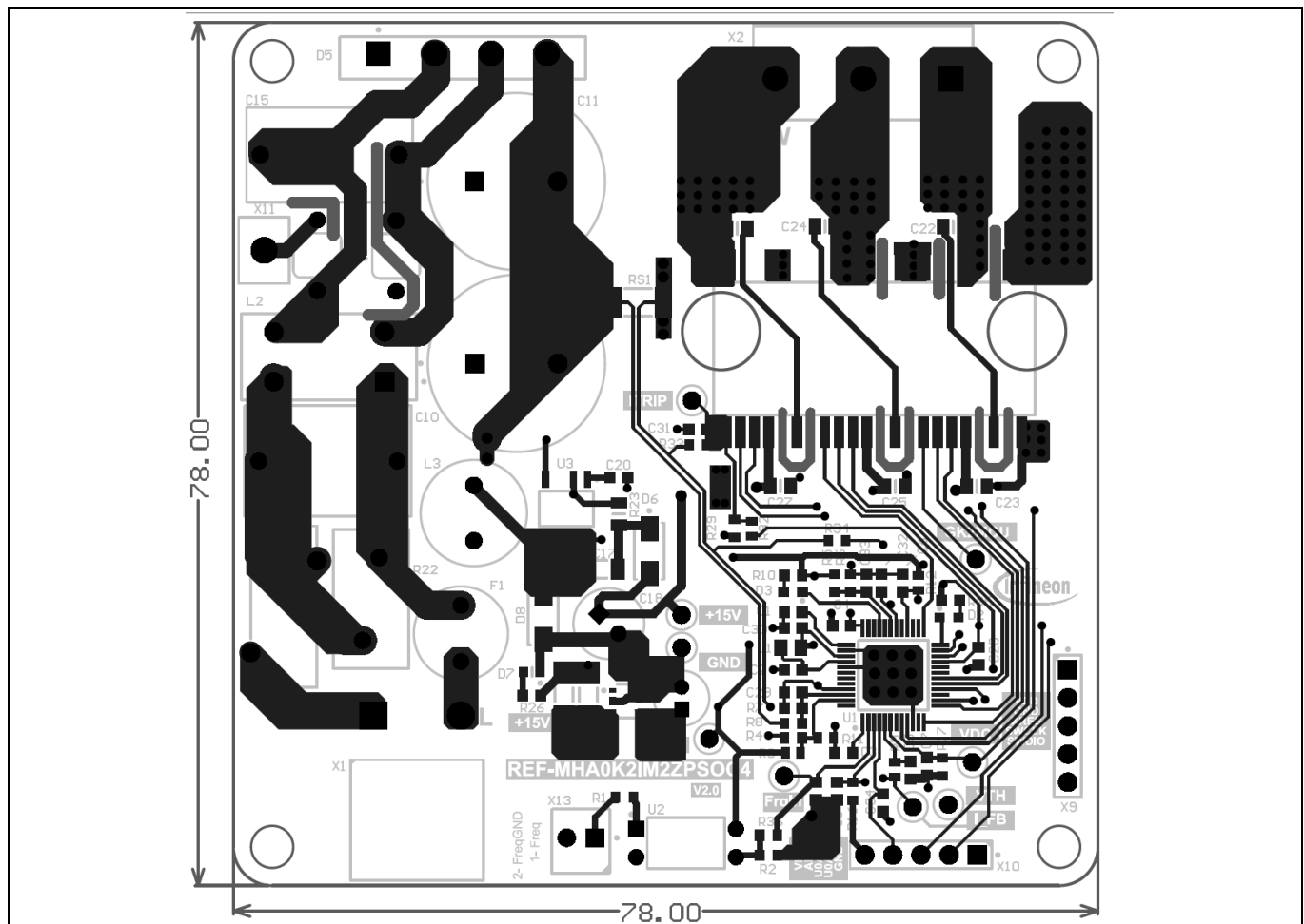
Figure 15 Top view of the board
