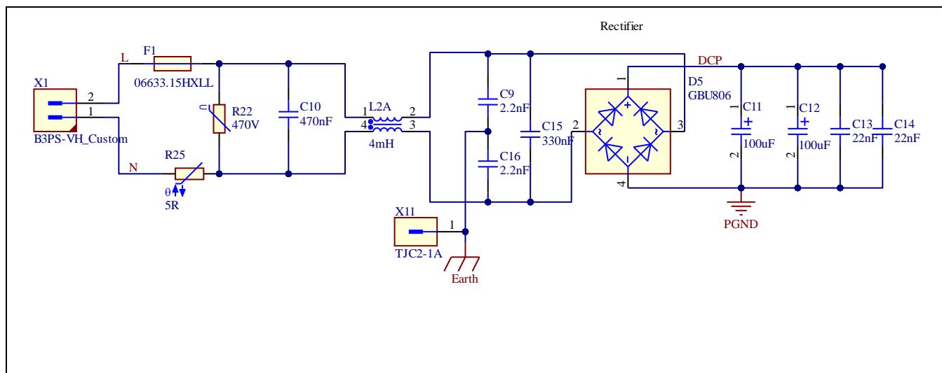
Figure 13 Schematic from the AC input connector to the rectified DC bus voltage
