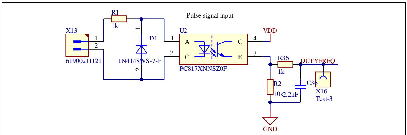
Figure 12 Frequency interface circuit
