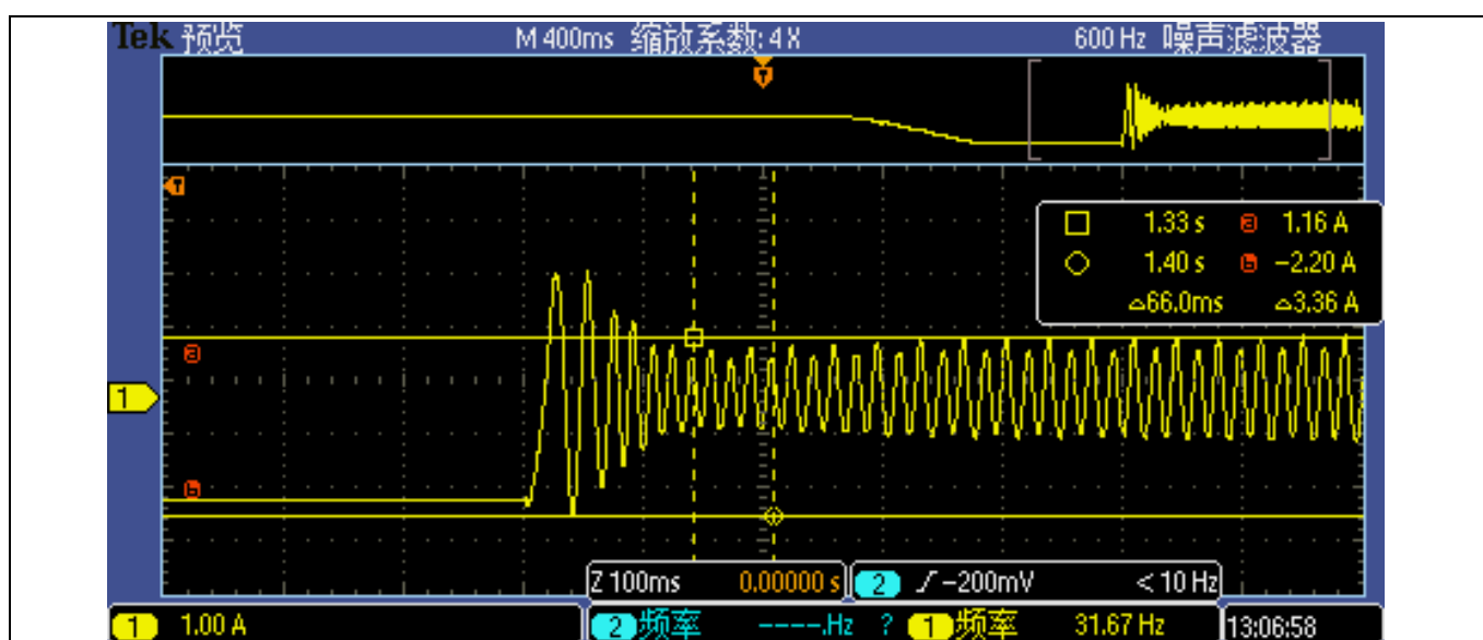
Figure 17 Start-up waveform of fridge at heavy load
