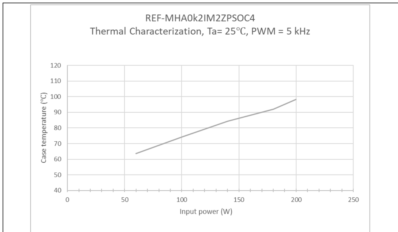
Figure 21 REF-MHA0K2IM2ZPSOC4 thermal characterization case temperature – input power, t_a = 25^{\circ}\text{C} , PWM = 5 kHz
