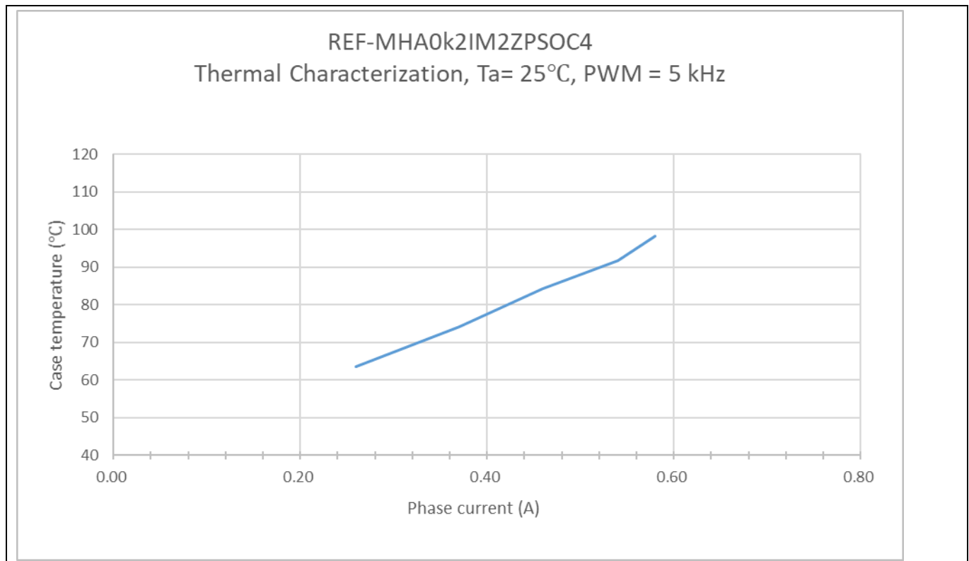
Figure 22 REF-MHA0K2IM2ZPSOC4 thermal characterization, case temperature - motor phase current, t_a = 25^\circ\text{C} , PWM = 5 kHz
