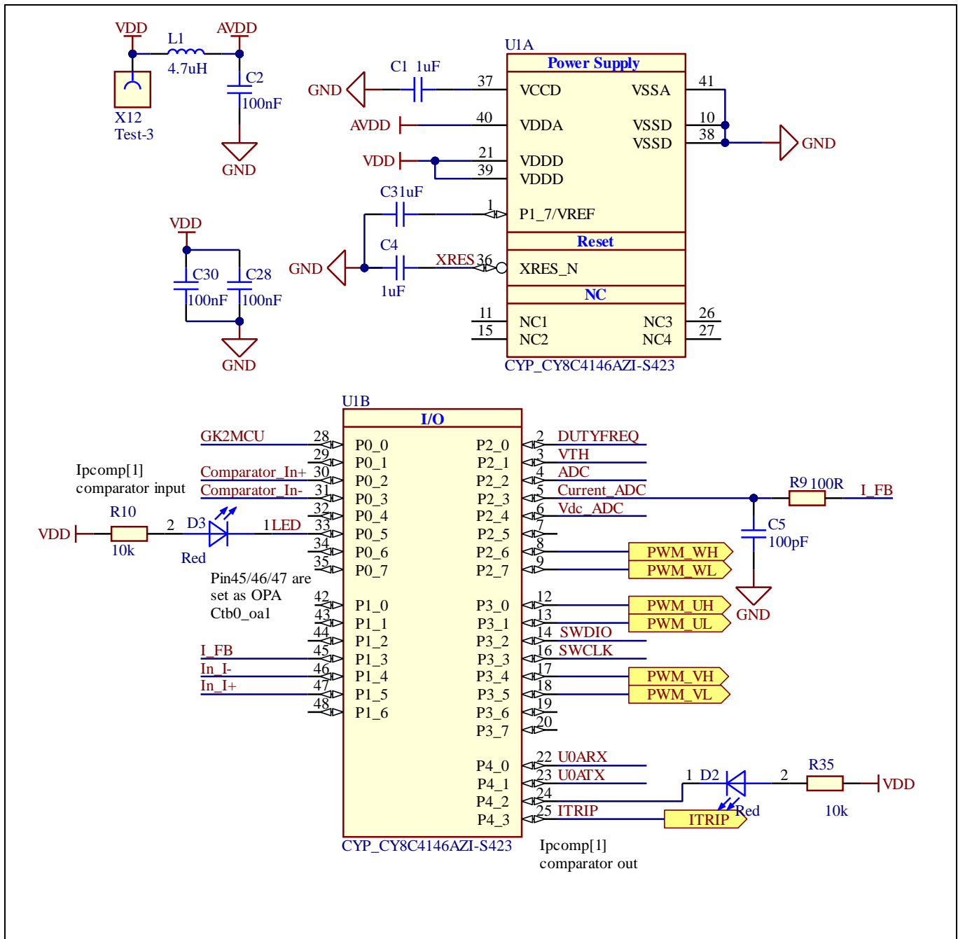
Figure 5 Schematic diagram of PSoC4 MCU
