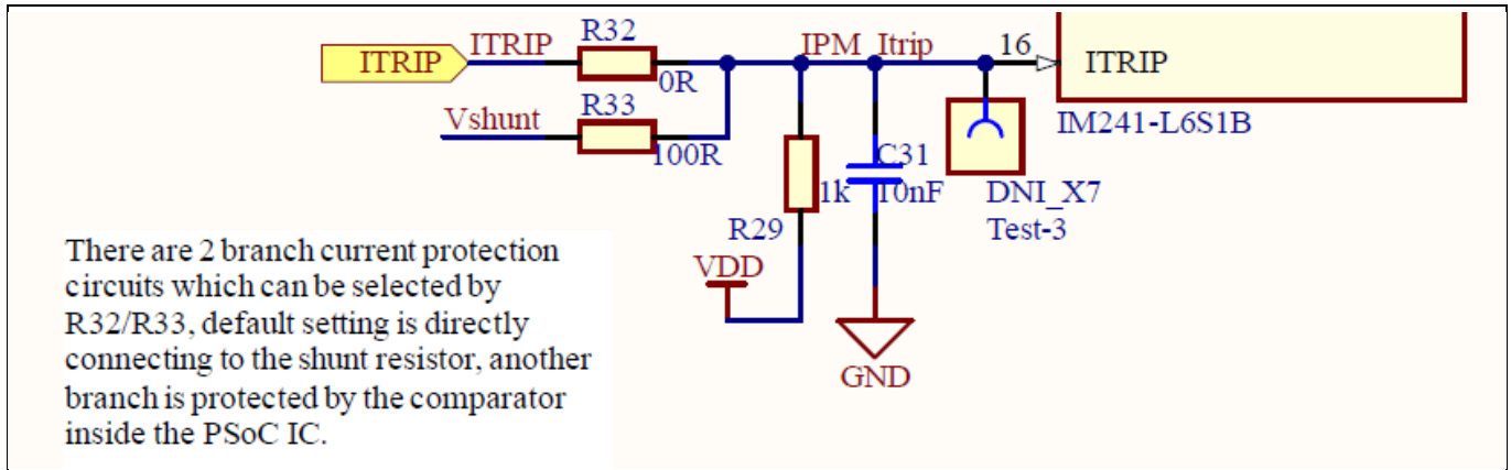
Figure 11 Hardware overcurrent circuit at pin VFO
