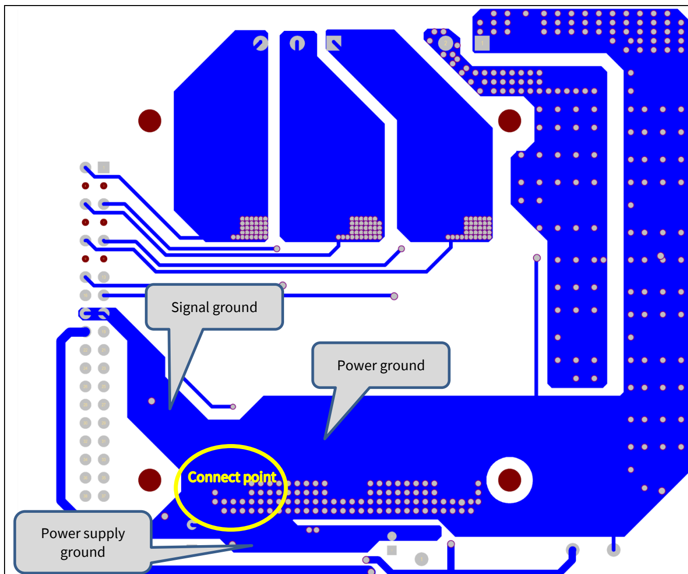
Figure 18 Bottom layer
