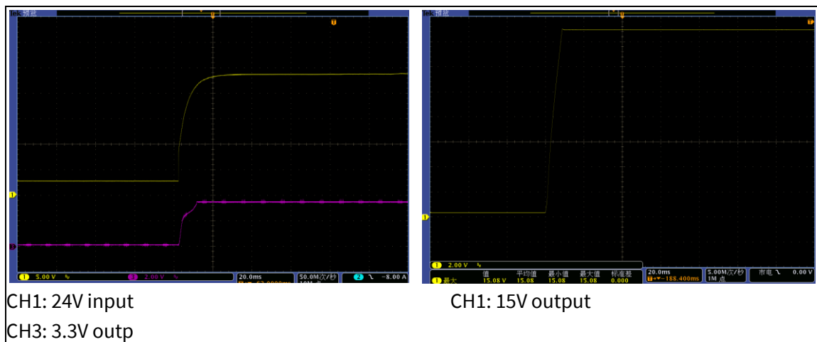
Figure 20 Aux. power supply start up at 24 V DC input
